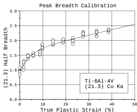
Figure 3 – Dependence of (21.3) peak breadth on “cold work” expressed as true plastic strain for Ti-6Al-4V. Samples were prepared in compression with multiple measurements shown. The K\alpha_1 peak breadth corresponding to 10% cold work is indicated.
