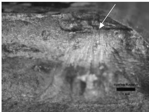
Figure 10 – Subsurface fatigue origin below the compressive layer produced by LPB.
