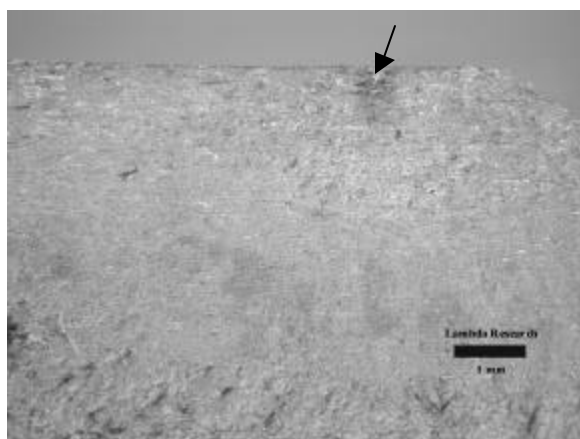
Figure 8 – Typical surface fatigue initiation site on machined 7075-T6 in active corrosion fatigue.
