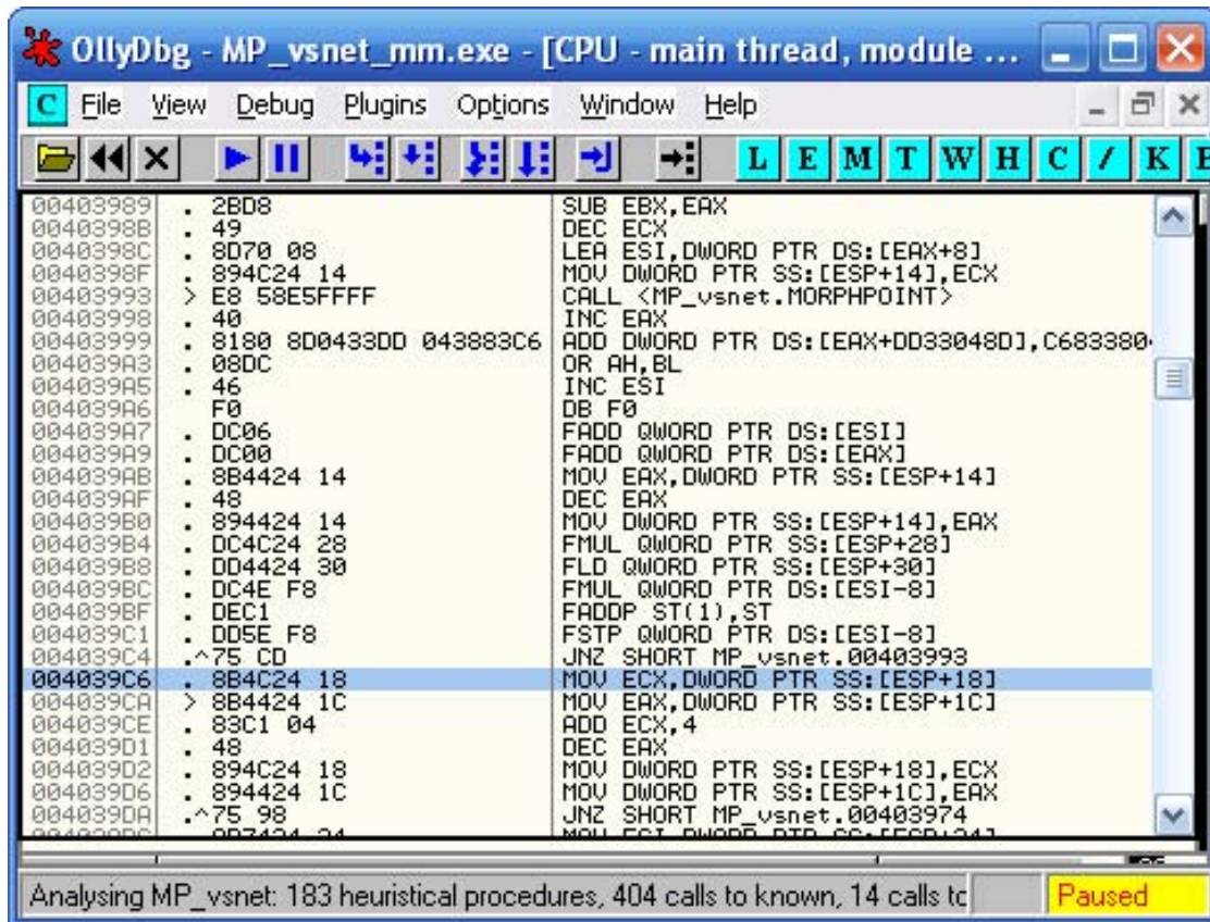
Figure 5.19. Using the analysis tool in OllyDbg after morph occurs
