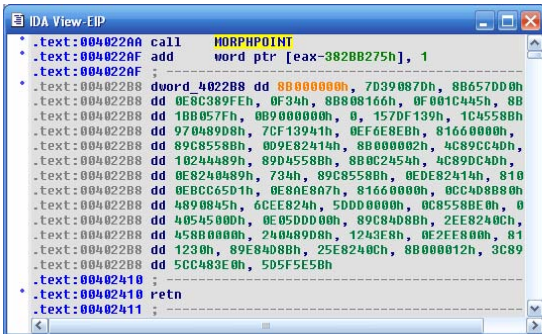
Figure 5.16. IDA Pro opens an executable that utilizes storage metamorphism
