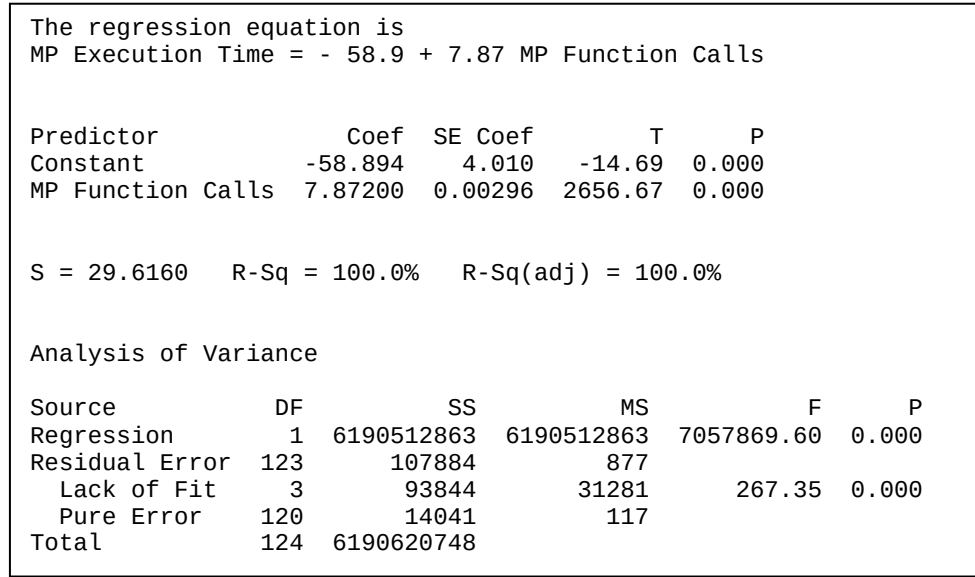
Figure A.19. Regression model generated by VSNET SMM benchmark program
