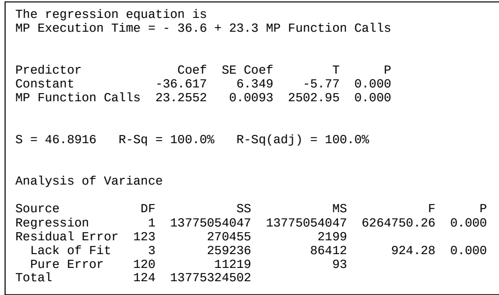
Figure A.21. Regression model generated by VSNET LU benchmark program
