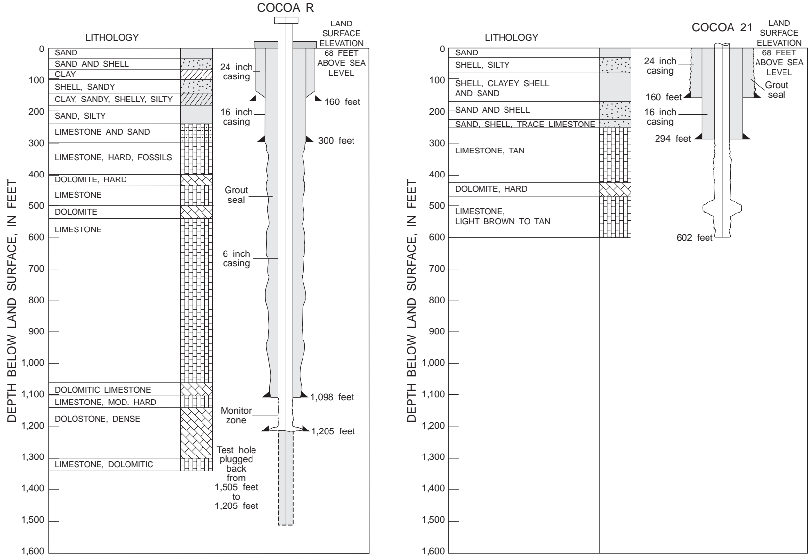
Figure 22. Geohydrologic section showing well-completion data for well R and supply well 21.
