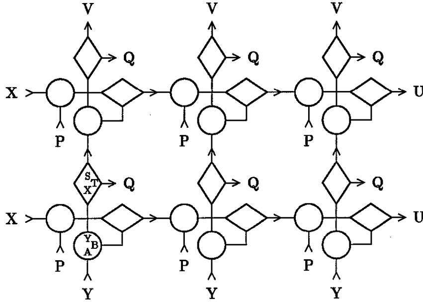
Figure 2: Building Block Interconnections for a One-way Mesh
