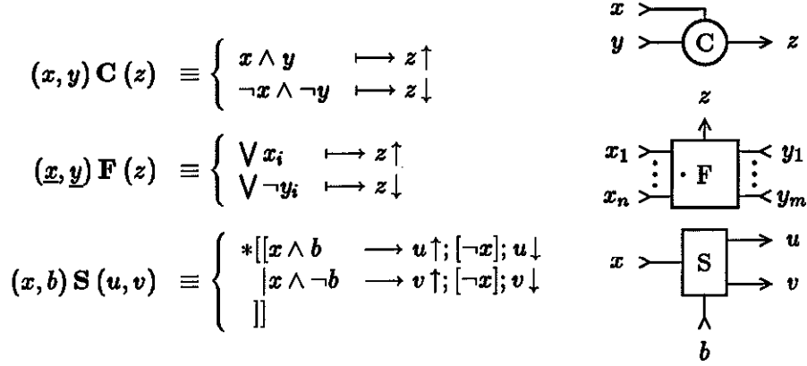
Figure 4: State-holding Operators
