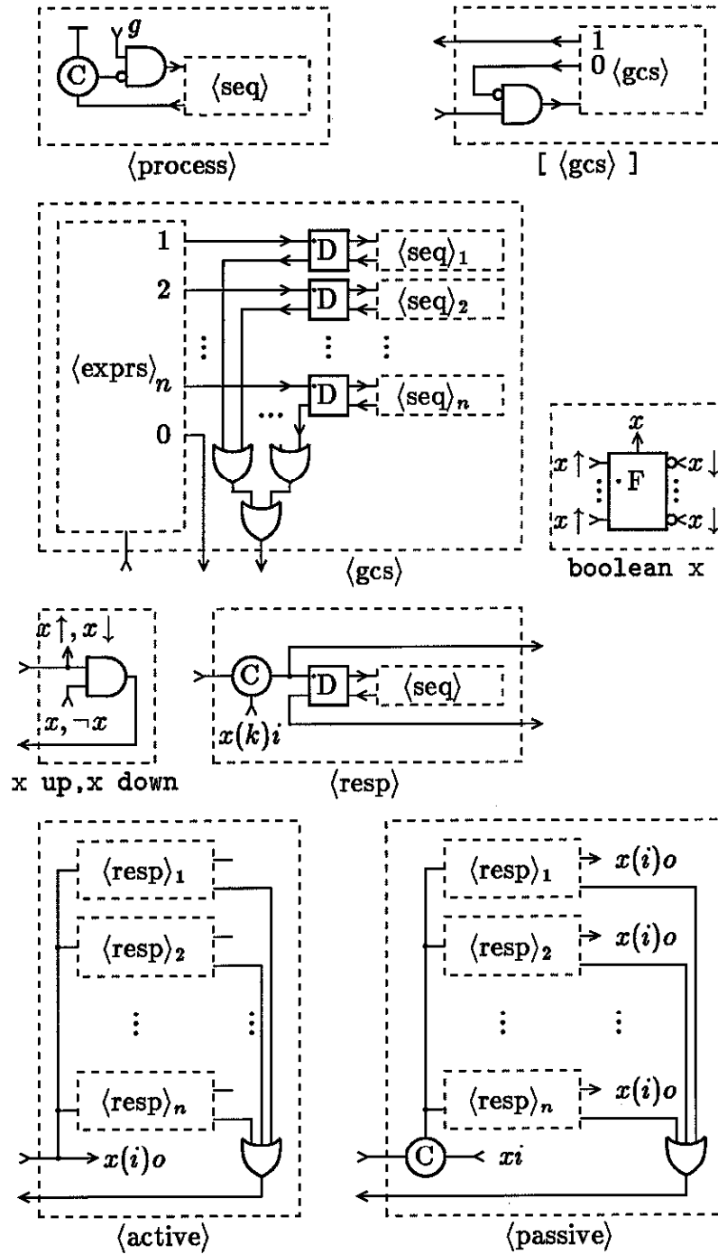
Figure 7: Circuits Implementing Statements
