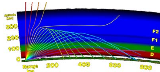
Figure 13: Ionospheric paths
