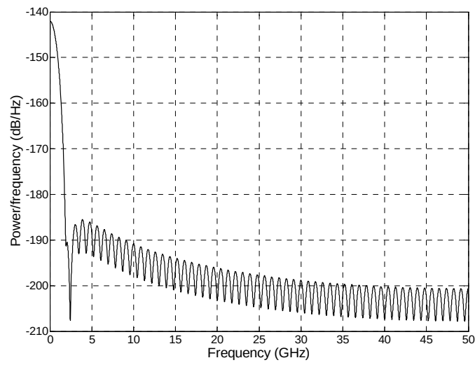
A.23 Down-converted received DSSS PSD
