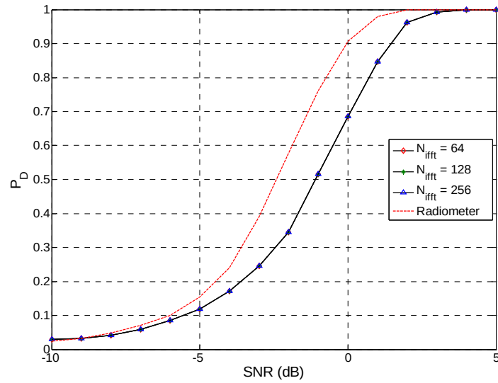
A.36 CTM detection performance for a BPF-D/C channelized receiver with M = 10 , 500MHz channels and varying number of IFFT points
