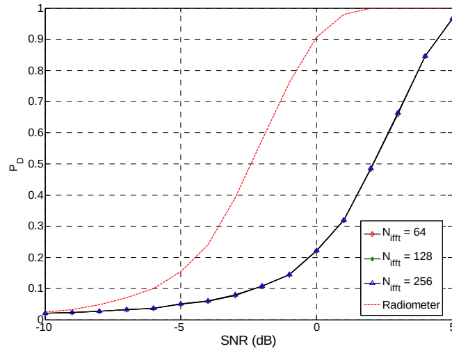
A.34 TTM detection performance for a BPF-D/C channelized receiver with M = 10 , 500MHz channels and varying number of IFFT points
