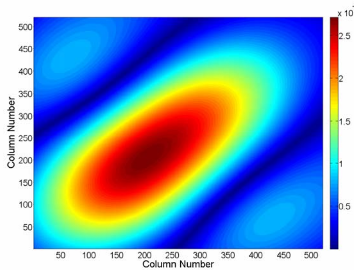
Figure 3.4 UWB cross temporal matrix (CTM) from a bandpass filtered, down-converting channelized receiver (BPF-D/C ChRx)
