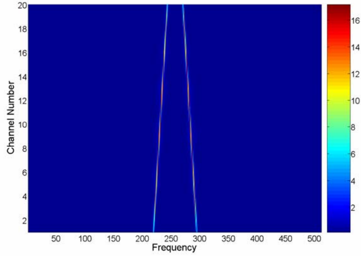
Figure 2.15 UWB: Spectral-spectral matrix (SSM) from channelized receiver
