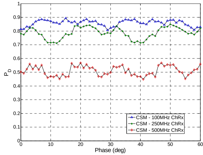
Figure 4.14 CSM detection performance versus mixer phase for a D/C channelized receiver using \text{SNR} = 0 dB with varying channel bandwidth [19]
