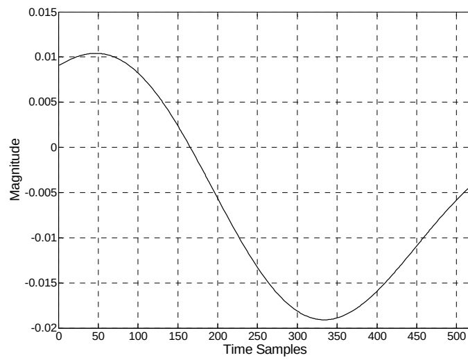
A.14 Down-converted received UWB pulse
