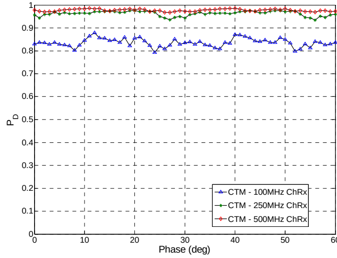
Figure 4.10 CTM detection performance versus mixer phase for a D/C channelized receiver using SNR = 0 dB with varying channel bandwidth [19]
