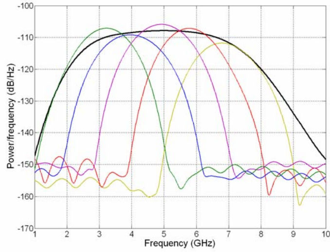
A.17 PSD comparison of H_{RF} and BPF_{1-M} for UWB using 1 GHz channels
