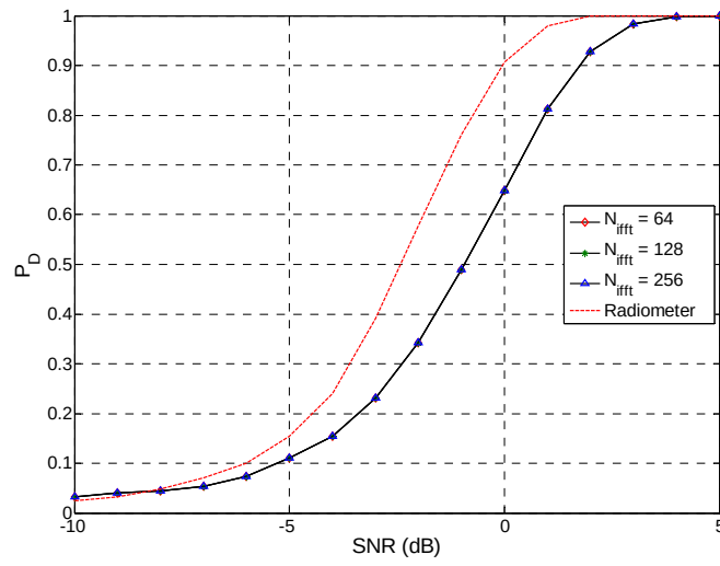
A.35 CTM detection performance for a BPF-D/C channelized receiver with M = 50 , 100MHz channels and varying number of IFFT points
