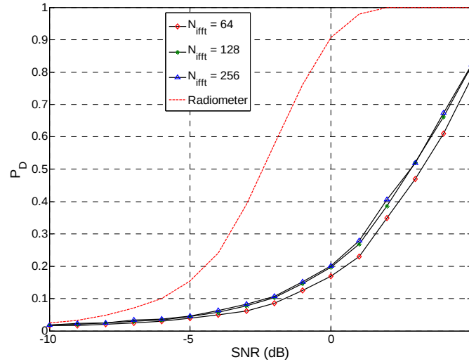
A.33 TTM detection performance for a BPF-D/C channelized receiver with M = 50 , 100MHz channels and varying number of IFFT points
