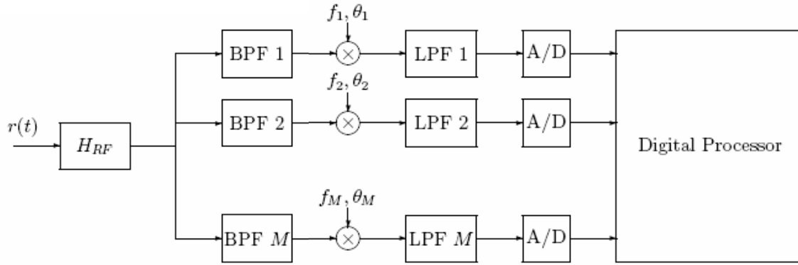
Figure 3.1 Bandpass filtered, D/C channelized receiver (BPF-D/C ChRx)
