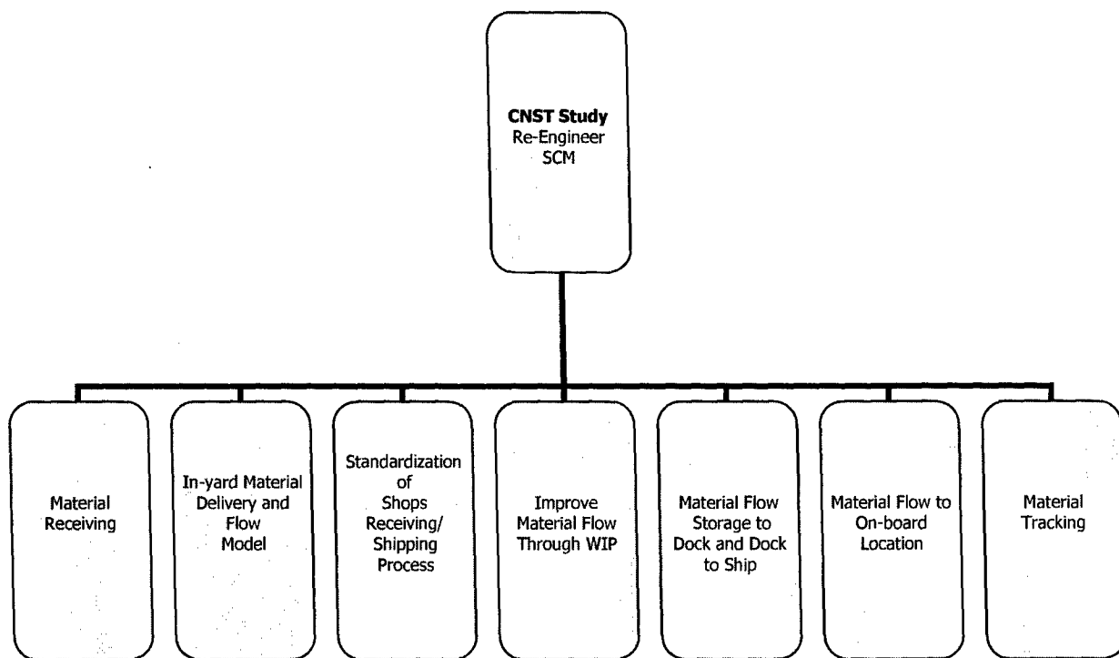
Project Structure
