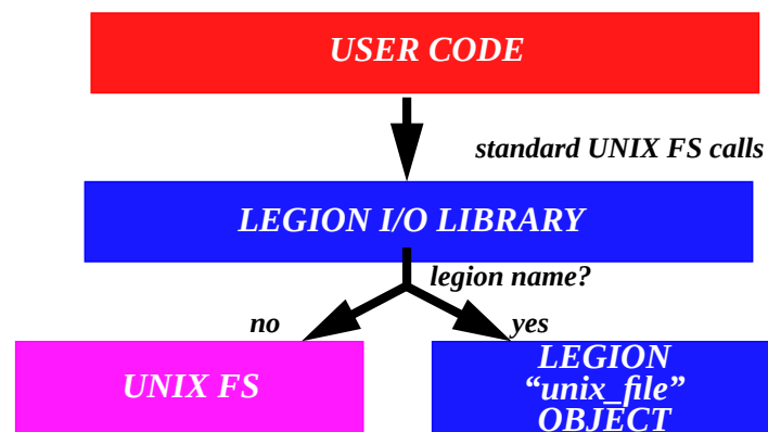
Figure 1 Emulation of the stdio interface allows applications to use the Legion federated file system capabilities without modification.
