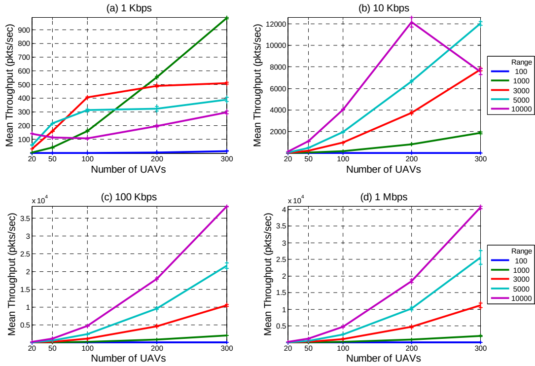
Figure 47. Mean Throughput versus Number of UAVs
