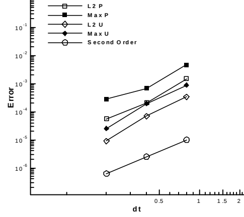
Fig. 3 Time accuracy test, decaying vortices, q=0.5
