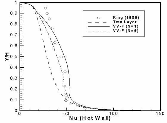
Fig.8 Local Nusselt number distributions
