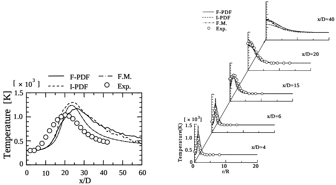
Fig.3 Axial profiles of temperature along the center axis.
