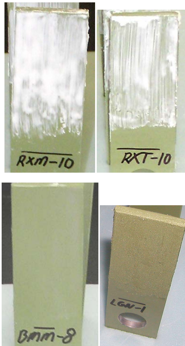
Figure 10. Selected phase 1 coated coupons prior to testing (clockwise from top left): Rain-X with maximum MP-55, Rain-X with typical MP-55, NAPA lithium grease with Knox gelatin, and Braycote 601EF with maximum MP-55 on an abraded surface.
