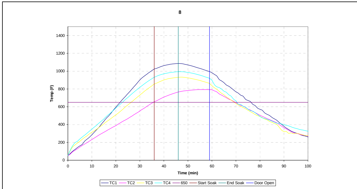
Figure 28: 120 mm shells-position A- Burners off during soak
