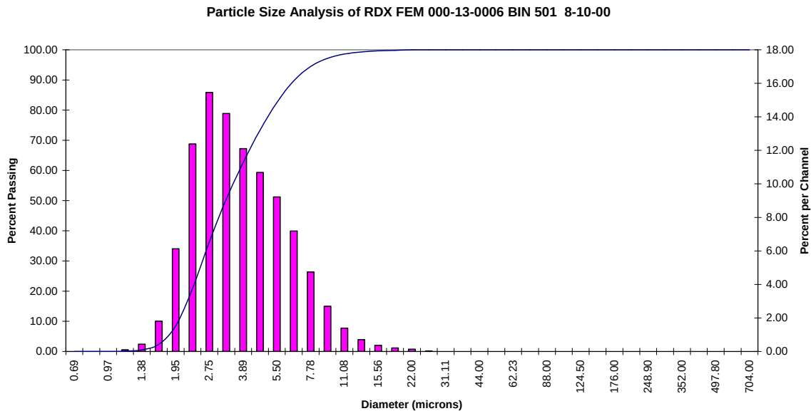
Figure 16: RDX, lot FEM 000-13-0006 particle size distribution (outer layer).
