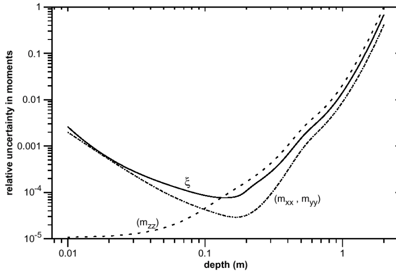
Figure 2.2.1: Relative rms polarizability uncertainty \xi as a function of sphere center depth below transmitter and receiver for a 6 cm radius steel sphere. Also, relative uncertainty in vertical moment dm_{zz}/dt (dashed), and in horizontal moments dm_{xx}/dt and dm_{yy}/dt (dotted).
