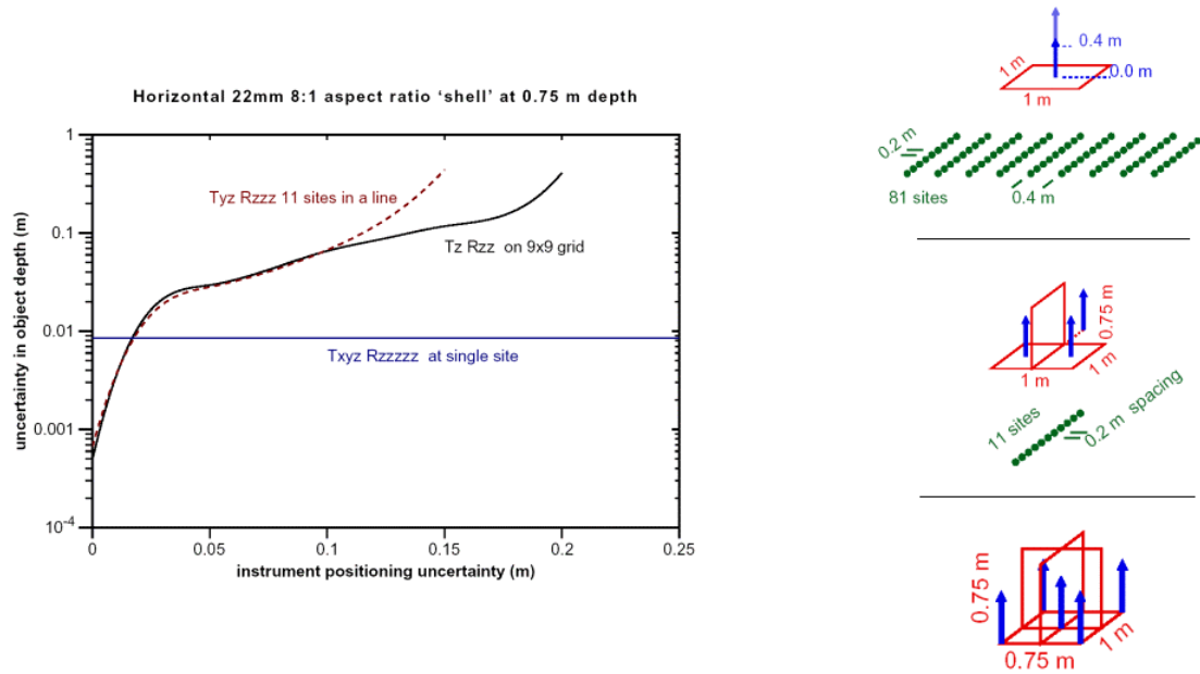
Figure 3.2.14: Relative rms depth uncertainty as a function of instrument location error for 22 mm 8:1 aspect ratio shell at 0.75 m depth at 610 \mu s after transmitter shut-off.
