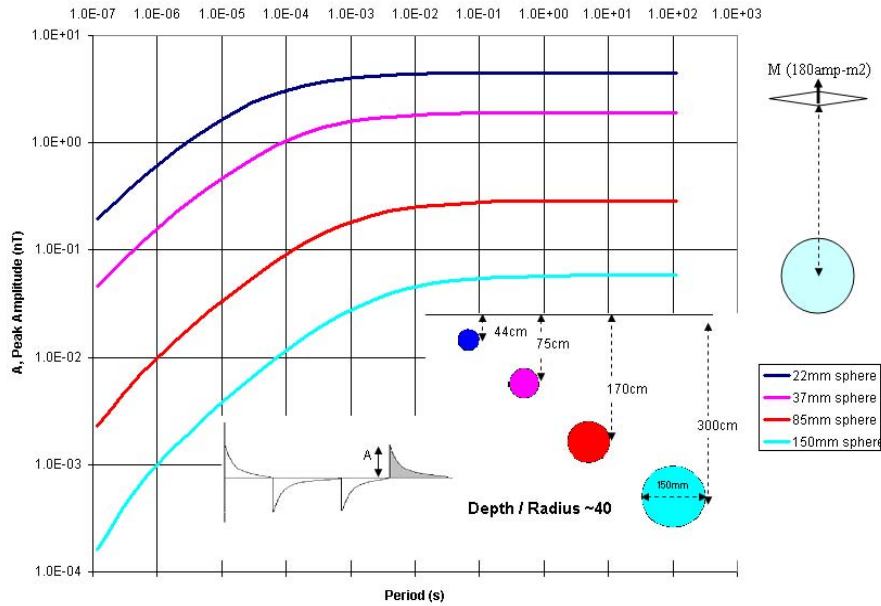
Figure 3.5.2: The amplitudes for four representative spheres at four different depths plotted as a function of repetition period.
