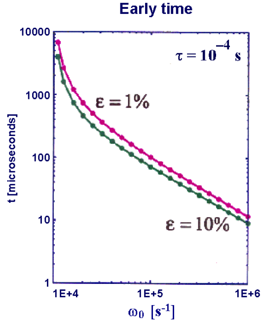
Figure 3.7.6: Earliest time of detection, to 1% or 10% accuracy for 100 \mu\text{s} target.
