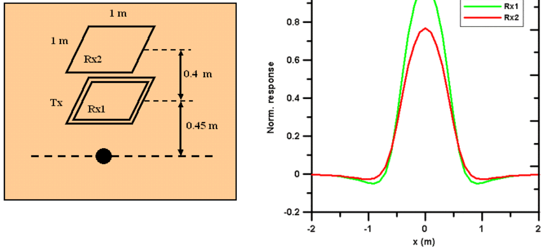
Figure A.1.2.1: EM-61 simulation.
