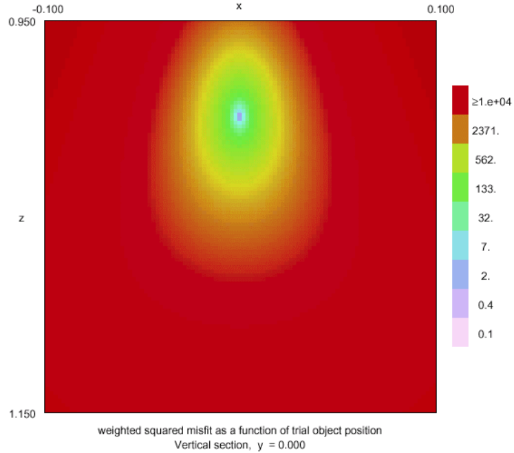
Figure 2.1.2: Squared data misfit \chi^2 as a function of candidate object center position r_0 , for 1 \text{ m}^2 square transmitter loop, 2 coaxial vertical dipole receiver system sited on a 9 \times 9 grid, centered 1 m above a 12 cm steel sphere (detail).
