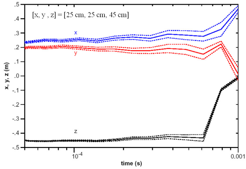
Figure 4.3.5a: Inversion results for the position of 9 inch (23 cm) steel ellipsoid with offset.
