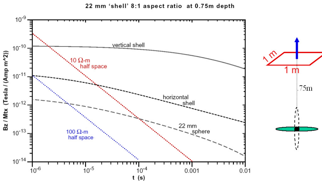
Figure 3.3.10: Amplitude of magnetic field response for 22 mm sphere, horizontal and vertical shells 8:1 aspect ratio at the depth of 0.75 m as a function of time together with responses for 10 \Omega -m and 100 \Omega -m half-space.
