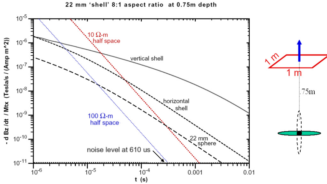
Figure 3.3.9: Amplitude of dB/dt response for 22 mm sphere, horizontal and vertical shells 8:1 aspect ratio at the depth of 0.75 m as a function of time together with responses for 10 \Omega -m and 100 \Omega -m half-space.
