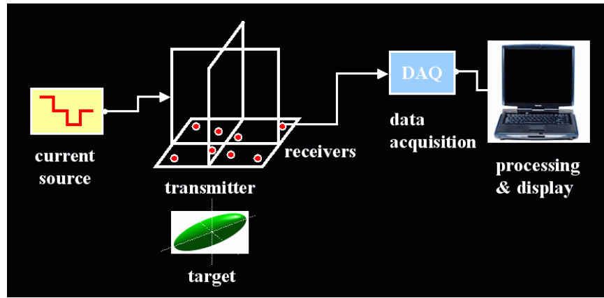
Figure 1.3.5: Schematics of the bench test acquisition setup.
