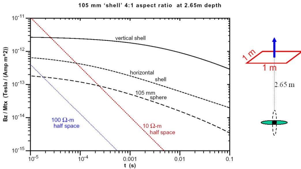
Figure 3.3.12: Amplitude of magnetic field response for 105 mm sphere, horizontal and vertical shells 4:1 aspect ratio at the depth of 2.65 m as a function of time together with responses for 10 \Omega -m and 100 \Omega -m half-space.
