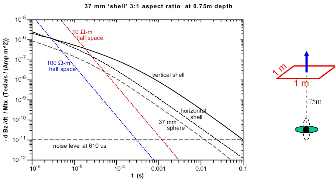
Figure 3.3.7: Amplitude of dB/dt response for 37 mm sphere, horizontal and vertical shells 3:1 aspect ratio at the depth of 0.75 m as a function of time together with responses for 10 \Omega -m and 100 \Omega -m half-space.
