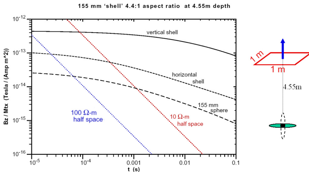
Figure 3.3.14: Amplitude of magnetic field response for 155 mm sphere, horizontal and vertical shells 4.4:1 aspect ratio at the depth of 4.55 m as a function of time together with responses for 10 \Omega\text{-m} and 100 \Omega\text{-m} half-space.
