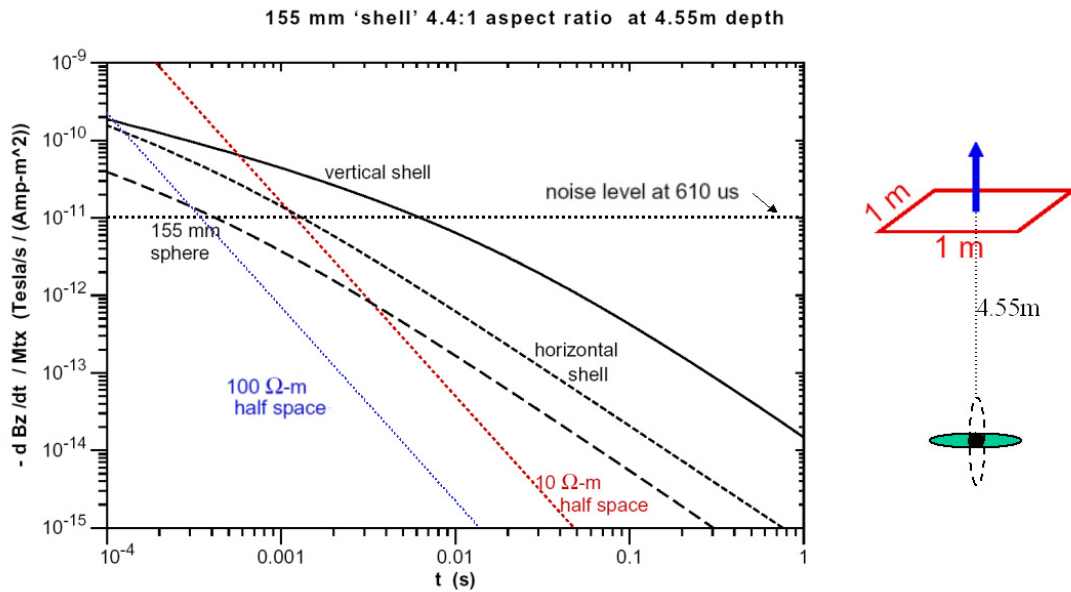
Figure 3.3.13: Amplitude of magnetic field response for 155 mm sphere, horizontal and vertical shells 4.4:1 aspect ratio at the depth of 4.55 m as a function of time together with responses for 10 \Omega\text{-m} and 100 \Omega\text{-m} half-space.
