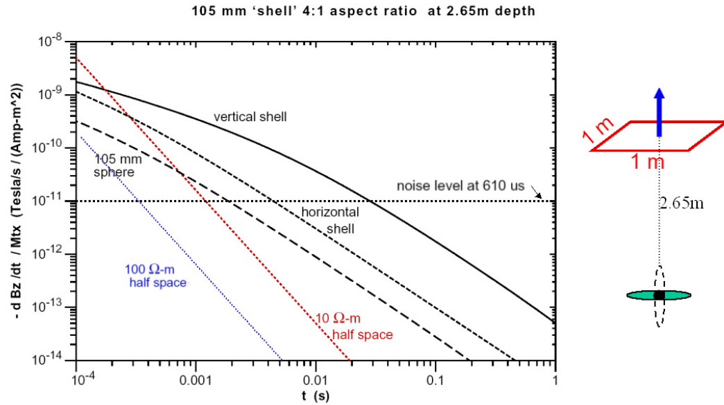
Figure 3.3.11: Amplitude of dB/dt response for 105 mm sphere, horizontal and vertical shells 4:1 aspect ratio at the depth of 2.65 m as a function of time together with responses for 10 \Omega -m and 100 \Omega -m half-space.
