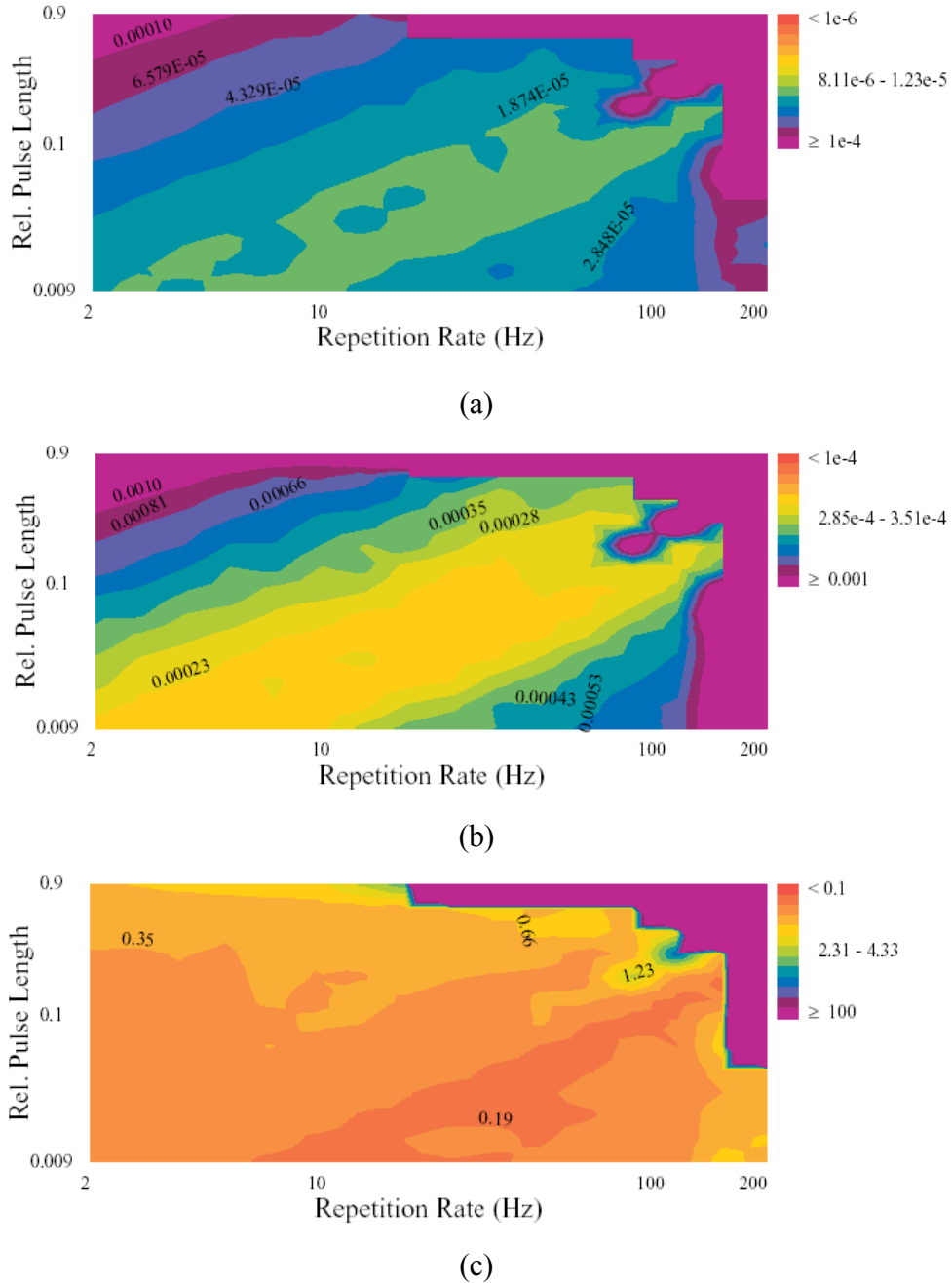
Figure 3.5.4: Uncertainties in (a) \log(r) , (b) \log(\sigma/\mu) , and (c) \log(\sigma\mu) for 160 mm sphere, resonant frequency f_0 = 3.2 kHz, and critically damped receiver.
