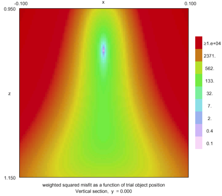
Figure 2.1.1: Squared data misfit \chi^2 as a function of candidate object center position r_0 , for 1 \text{ m}^2 square transmitter loop, concentric vertical dipole receiver system sited on a 9 \times 9 grid, centered 1 m above a 12 cm steel sphere (detail).
