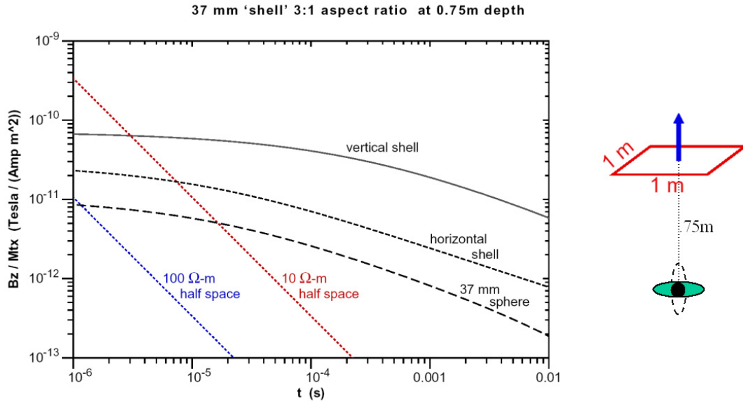
Figure 3.3.8: Amplitude of magnetic field response for 37 mm sphere, horizontal and vertical shells 3:1 aspect ratio at the depth of 0.75 m as a function of time together with responses for 10 \Omega -m and 100 \Omega -m half-space.
