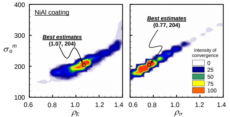
Fig. 9. Convergence maps generated after Kalman filter analysis. They show likely values of three known material properties.
