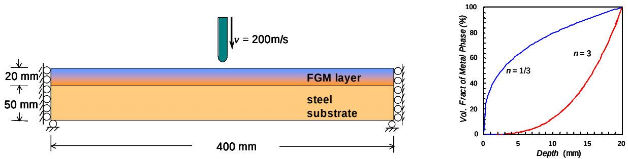
Fig. 6. Schematic of impact onto graded layer and two ceramic-metal different grading profiles through thickness.
