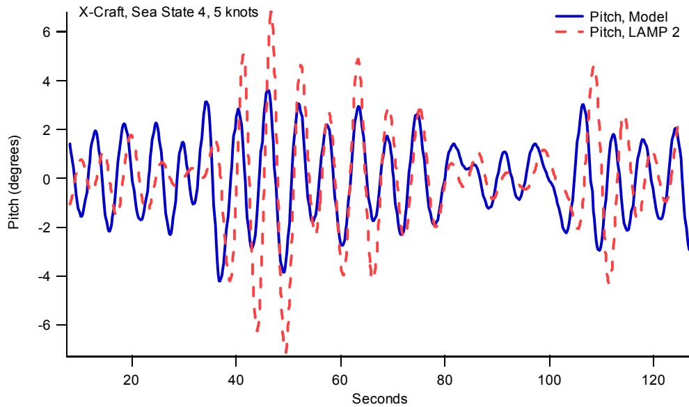
Figure 24: Comparison of Pitch Motion, Sea State 4, 5 knots, Head Seas
