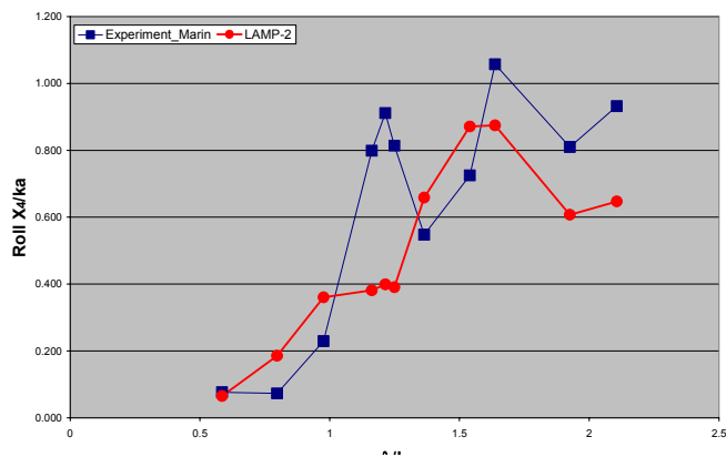
Figure 20: Roll Responses for \beta = 225^\circ & F_n = 0.30
