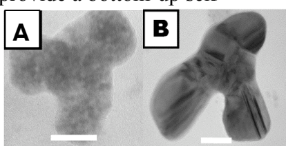
Fig. 8. TEM images of DNA-templated metallization of three-armed complexes with (A) copper or (B) silver; scale bars are 25 nm.
