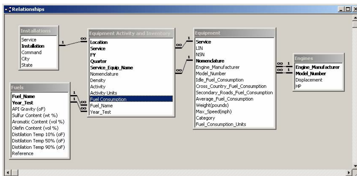
Figure 7. Overall database design.
