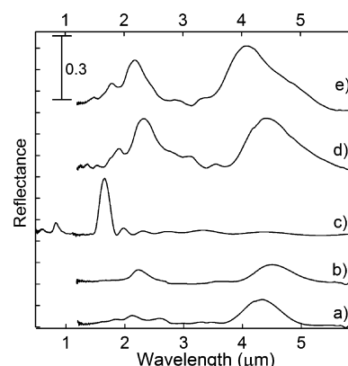
Figure 5. Reflectance spectra for a 3D microperiodic structure (8-layer structure, d = 2.8 \mu\text{m} ): a) Polymer woodpile; b) \text{SiO}_2 /polymer woodpile; c) \text{SiO}_2 hollow-woodpile; d) \text{Si/SiO}_2/\text{Si} hollow-woodpile; and e) \text{Si} hollow-woodpile after HF etch.
