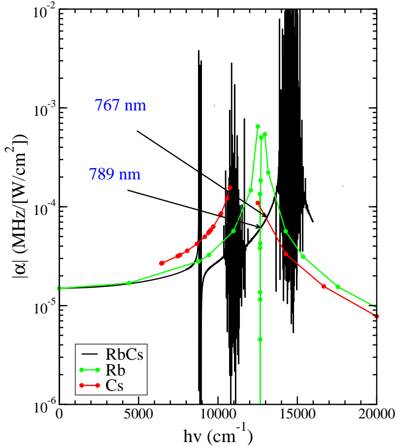
FIG. 3: Comparison of molecular and atomic dynamic polarizabilities of the ground states of RbCs (black curve), Rb (green curve) and Cs (red curve) as a function of laser frequency. Practical laser frequencies are indicated.
