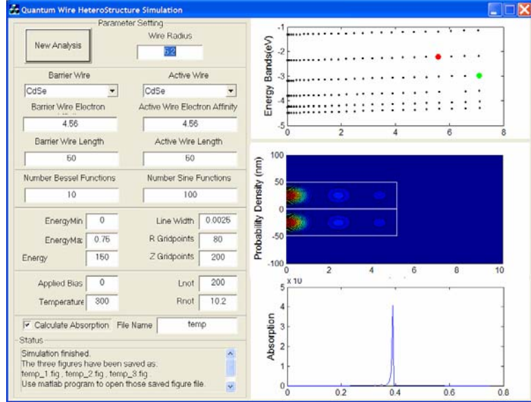
Fig. 4 The GUI for the FD algorithm to model QRIPs. This program was developed in this project and will allow for more sophisticated modeling of the QRIPs. It is being copyrighted and licensing opportunities are being explored.
