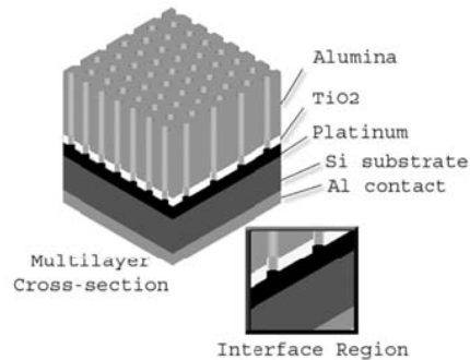
Figure 6: Left: Cross-section view of the alumina pores. The white bar is 1 micron. 17 Right: A schematic of the multilayer nanotemplate after anodization and voltage ramping to remove the \text{TiO}_2 layer at the base of the pores. Once the template fabrication is complete, the pores terminate at the Pt.
