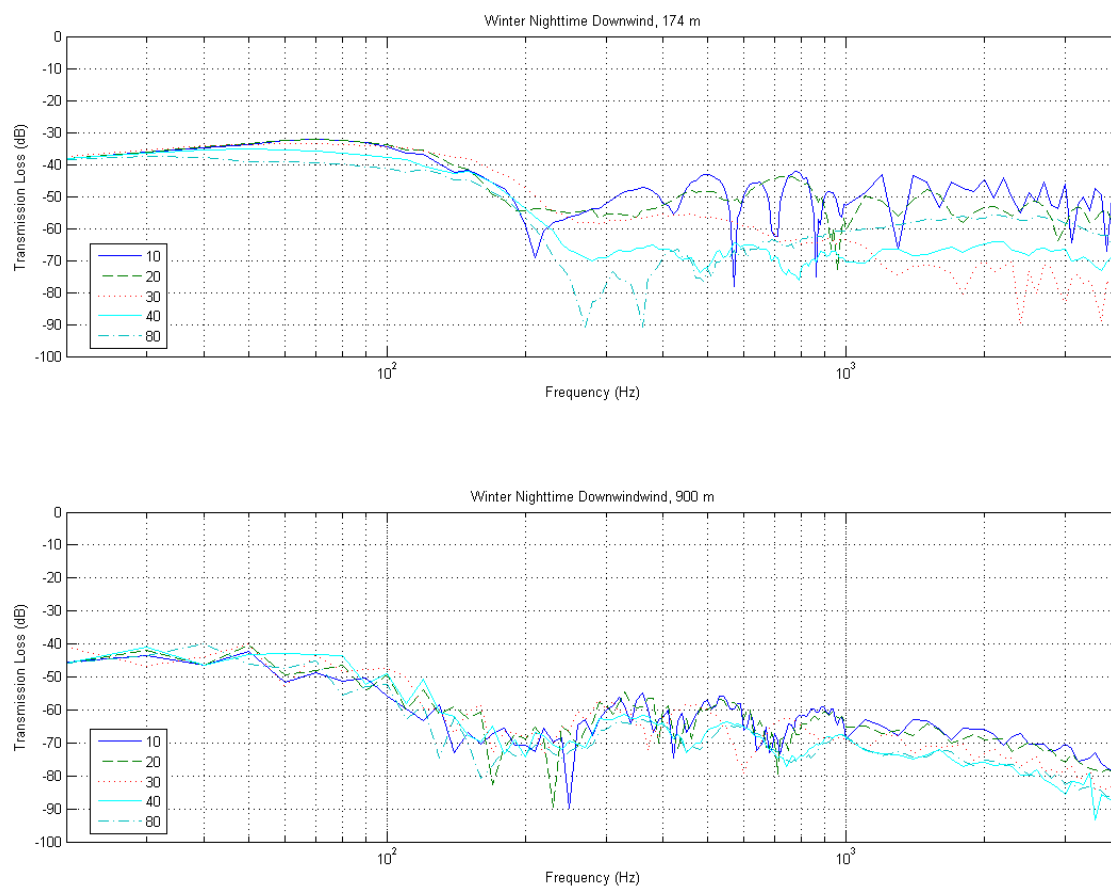
Figure 5. Winter Nighttime downwind cases, all forest stand ages, transmission loss of unweighted levels.
