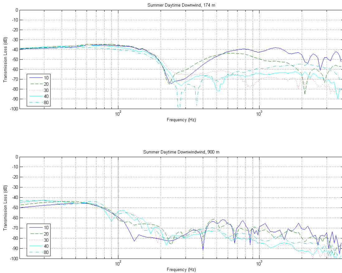
Figure 2. Summer Daytime downwind cases, all forest stand ages, transmission loss of unweighted levels.
