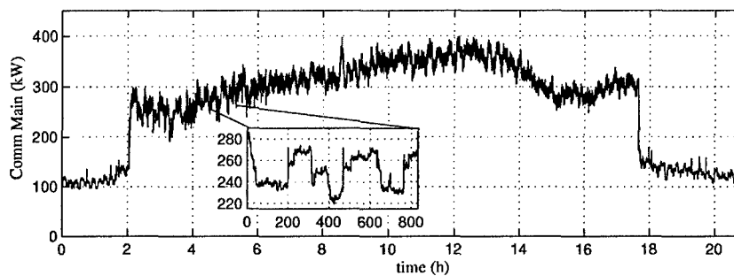
FIGURE 1: NILM Data from a Large Commercial Building
