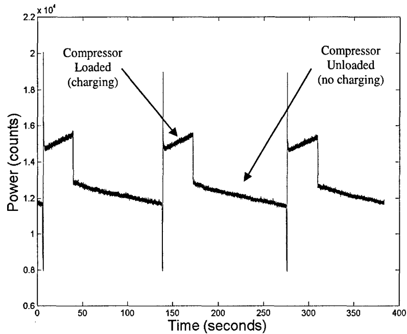
Figure 3-15: LPAC in Automatic 125PSIG Operation
