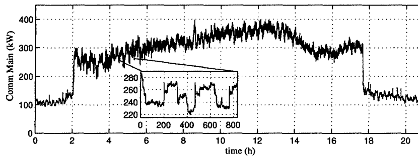
Figure 1-1: NILM Data from a Large Commercial Building
