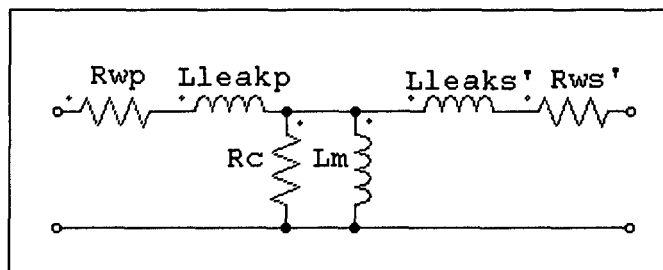
Figure 29: Inductive Coupler Parameters with Secondary Components Transformed
