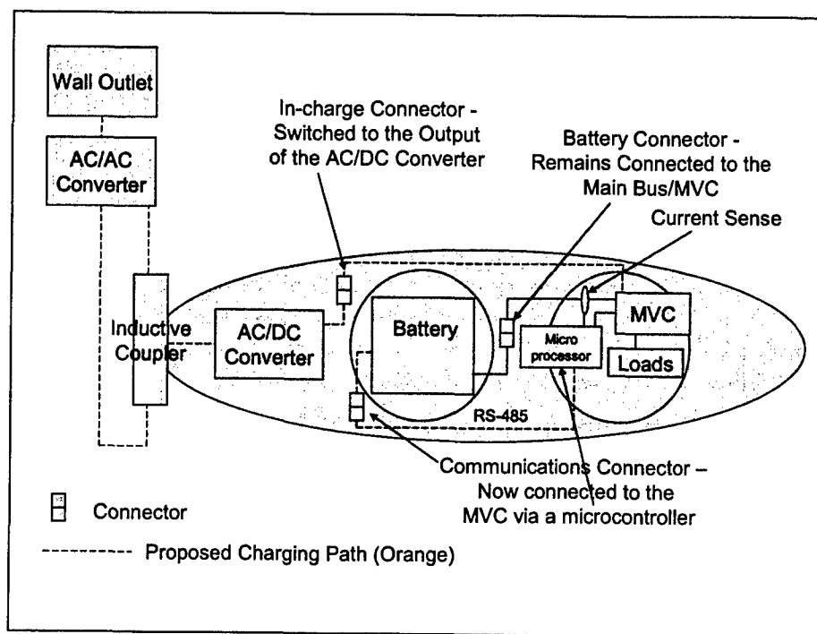
Figure 3: Proposed Charging Scheme
