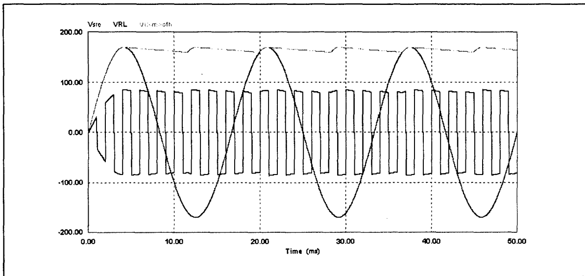
Figure 14: Half-bridge Waveforms
