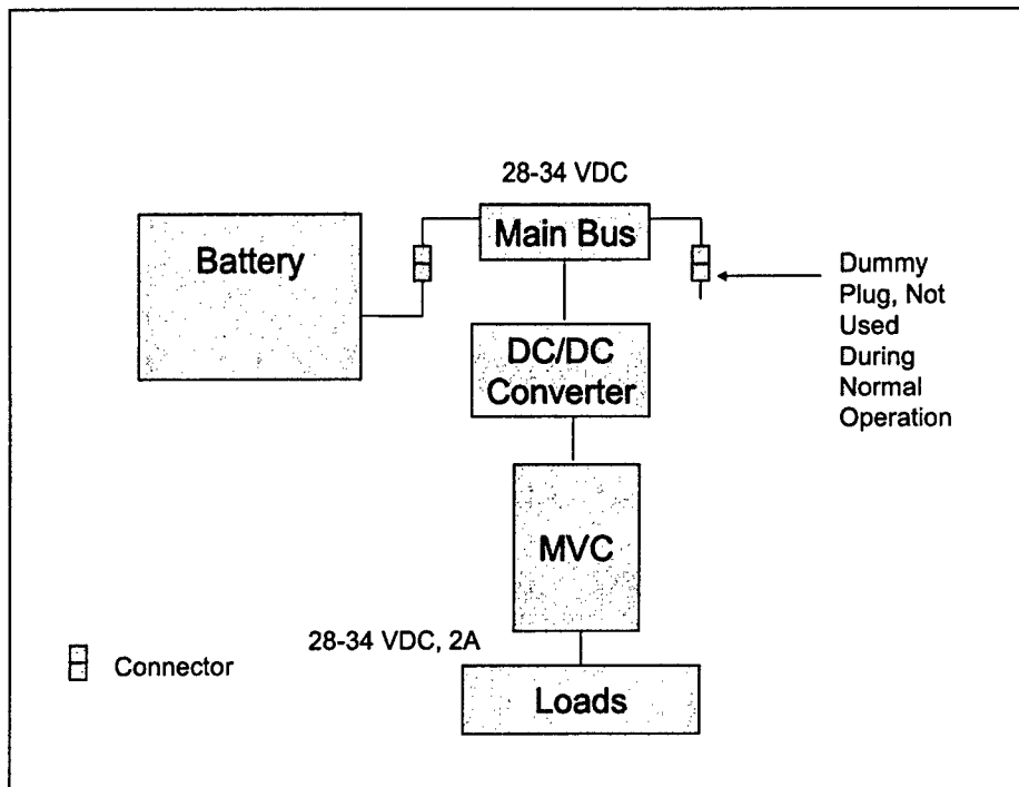
Figure 1: AUV Power Supply (Normal, Underway, Not Charging)
