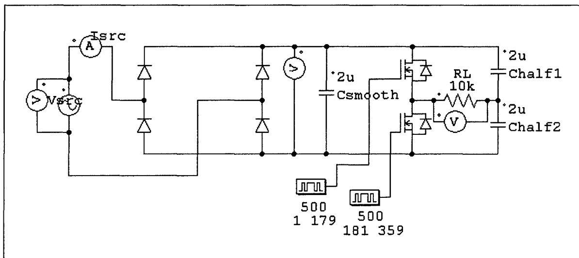
Figure 13: Half-bridge Circuit Diagram
