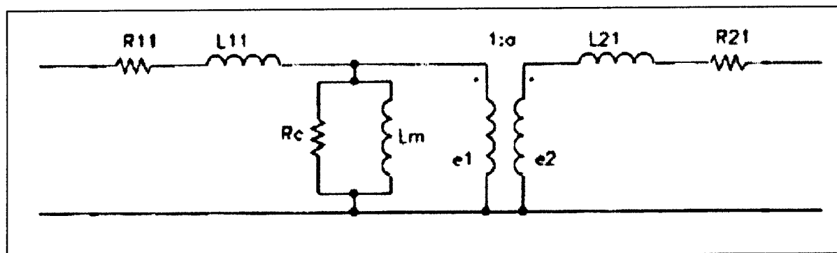
Figure 7: Simplified IEEE Equivalent Circuit [1]
