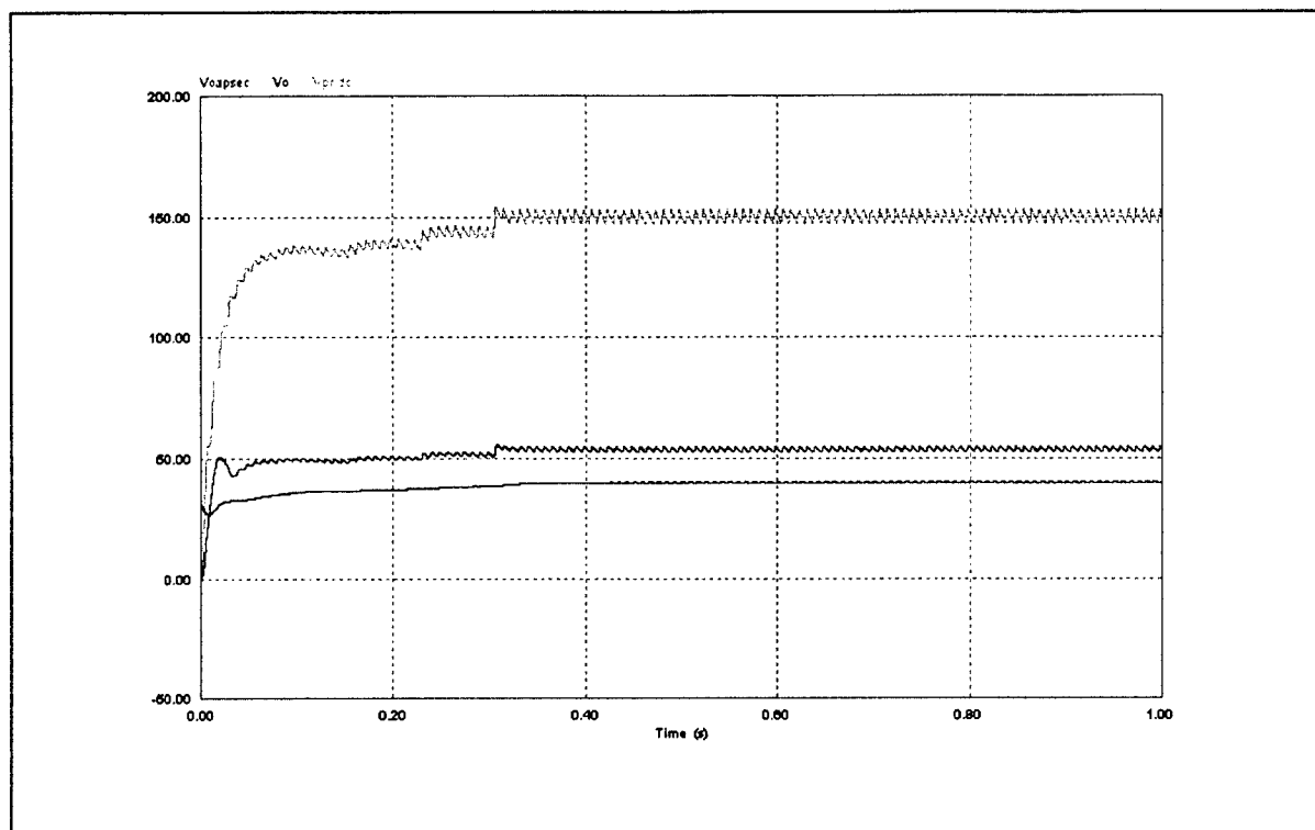
Figure 32: Simulation: I_{CHARGE}=15A , dV_O=52mV
