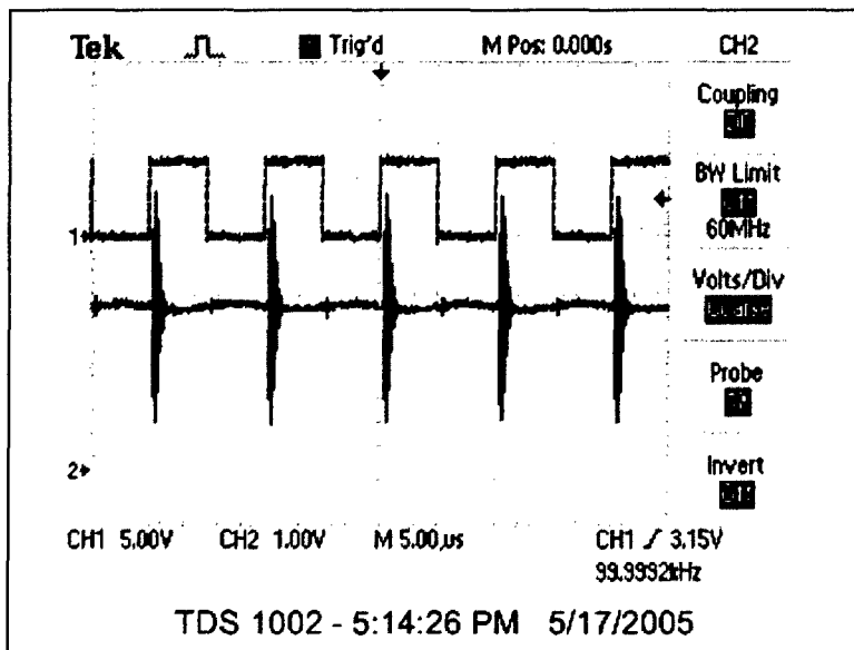
Figure 36: MOSFET Driver Input and "Buck" Converter Output Waveforms: V_{in}=6.2\text{VDC} , V_{out}=2.26\text{V} , d=0.5
