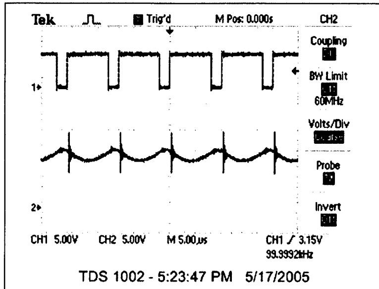
Figure 37: MOSFET Driver Input and "Buck" Converter Output Waveforms: V_{in}=12.7 VDC, V_{out}=9.2 V, d=0.8
