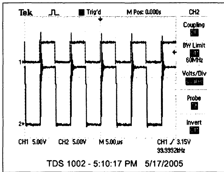
Figure 35: MOSFET Driver Input and Output Waveforms: V_{in}=6.2\text{VDC} , V_{out}=2.26\text{V} , d=0.5
