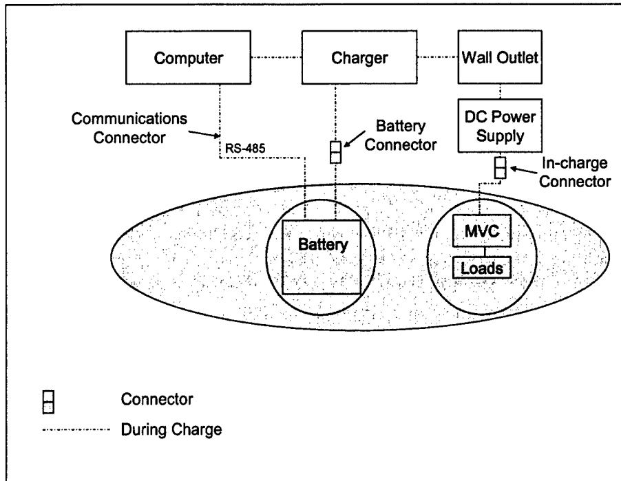
Figure 2: Current Battery Charge Scheme
