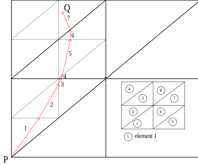
FIGURE 1: An example of in-element particle tracking
