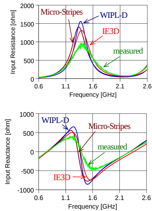
Figure 7 Input impedance of antenna No.2. L=88\text{mm} , d=38\text{mm} , g=2\text{mm}
