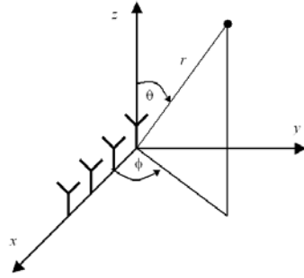
Fig. 6 , Geometry of the antenna array
