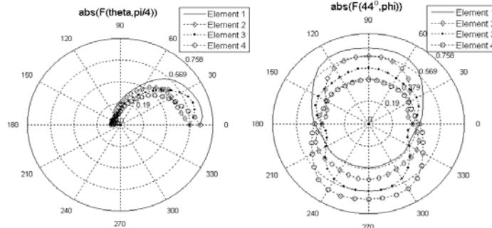
Fig. 4 element patterns of array Array1 at \phi=\pi/4 (left) and at \theta=44^\circ (right)
