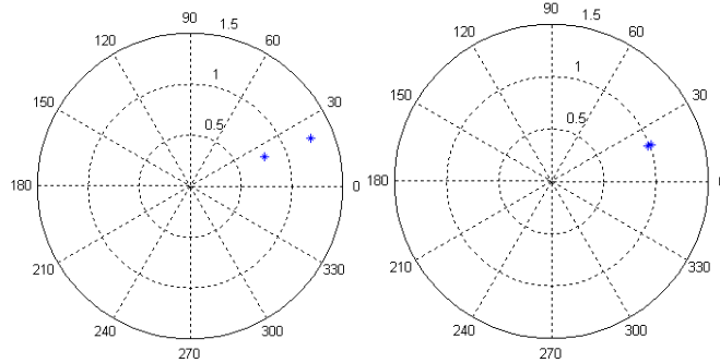
Fig. 7 DoA estimation roots using Array1 (left) and Array2 (right)
