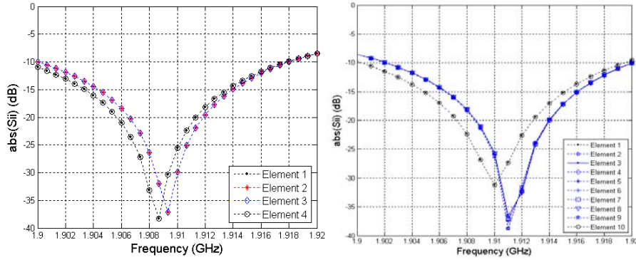
Fig. 3 Return loss of Array1 (left), Array2 (right)
