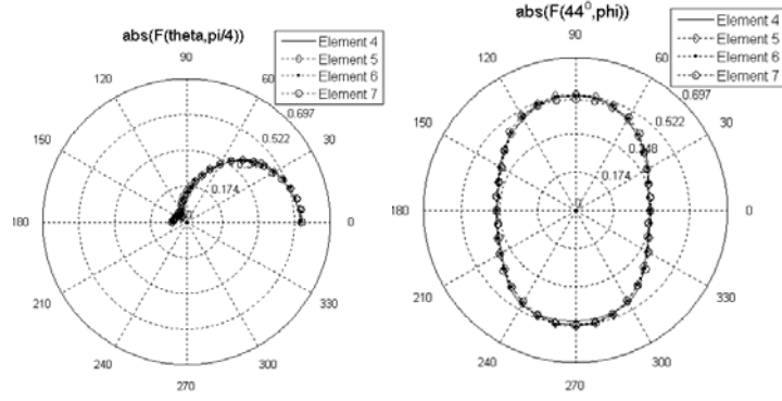
Fig. 5 Element patterns of the active 4 elements of Array2 at \varphi=\pi/4 and at \theta=44^\circ (right)
