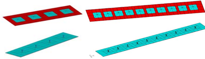
Fig. 2 A 4-element (left) and 10-element (right) array of patch antennas modeled in WIPL
