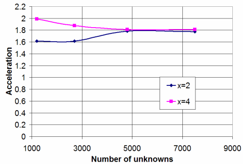
Figure 6: Acceleration in the case of dual processor run; x – number of tasks simultaneously assigned
