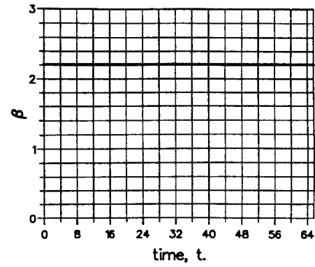
Figure 5.3.6 Algorithm P_1^{h,k} , the estimated convergence rate of \|\sigma - \sigma^h\|_{0,\Omega} with \beta , given by (5.3.1), obtained by considering h = 1, k = 0.1 and h = 0.5, k = 0.05 .
