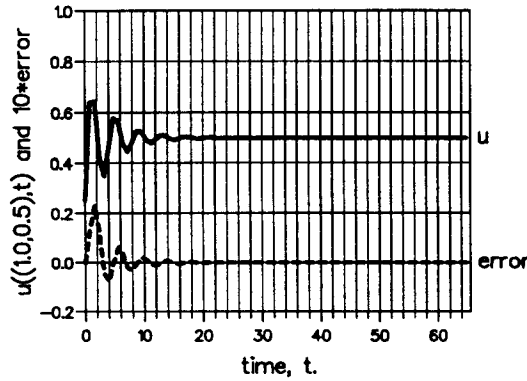
Figure 5.3.3 Algorithm P_2^{1,0.8} , the computed solution for (u_1^h(1, \frac{1}{2}))_r and the associated error. The discretization error tends to zero as the body force tends to a function of x only.
