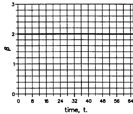
Figure 5.3.8 Algorithm P_1^{h,k} , the estimated convergence rate of \|\sigma - \sigma^h\|_{0,\Omega} with \beta , given by (5.3.1), obtained by considering h = \frac{1}{8}, k = 1.0 and h = \frac{1}{16}, k = 0.5 .
