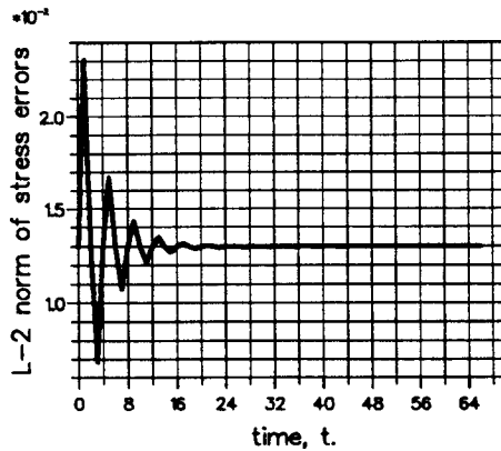
Figure 5.3.7 Algorithm P_1^{\frac{1}{4},1,0} , the computed value of \|\sigma - \sigma^h\|_{0,\Omega} . The discretization error tends to a constant as the body force tends to a function of x only.
