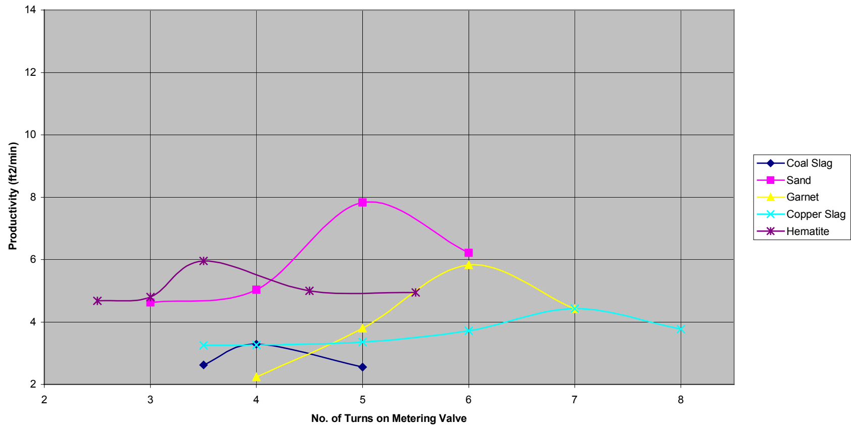
Productivity Data - 80 psi
