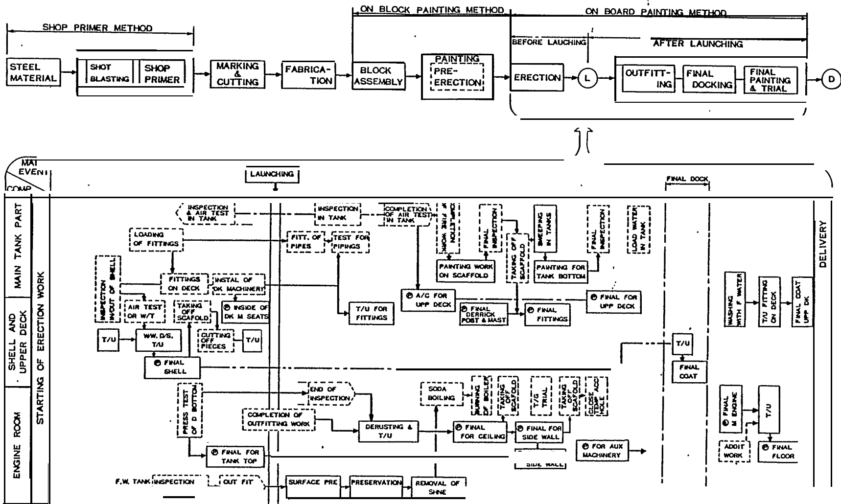
Figure 7-2: Sample On-Board Painting Procedure
