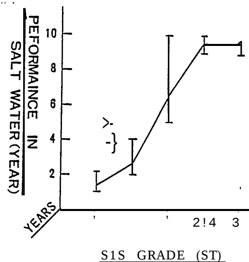
Figure 4-2: Chlorinated Rubber Paint Performance in Sea Water
