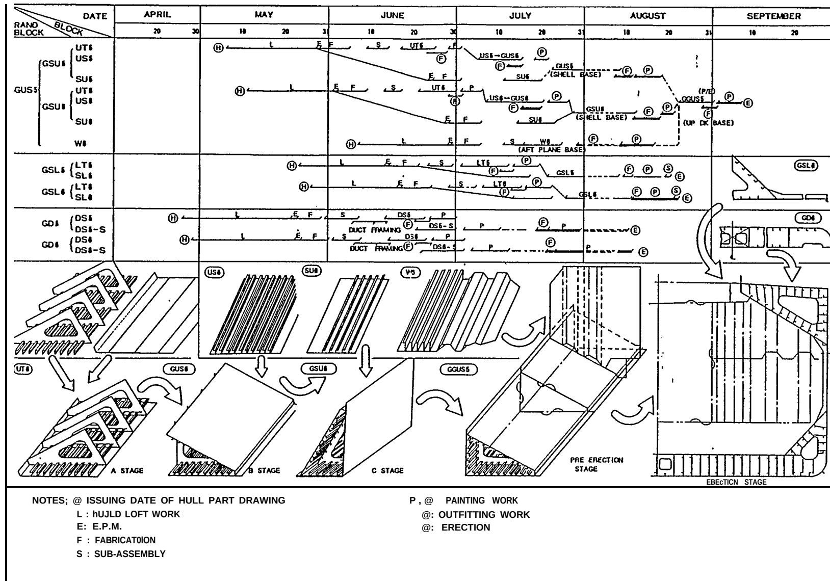
Figure 6-2: Painting Stages in a-Block Assembly Schedule
