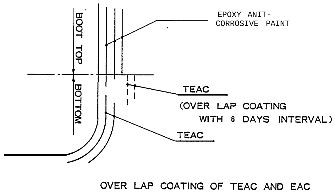
Figure 7-6: Overlap Coating of Two Kinds of Paint Material
