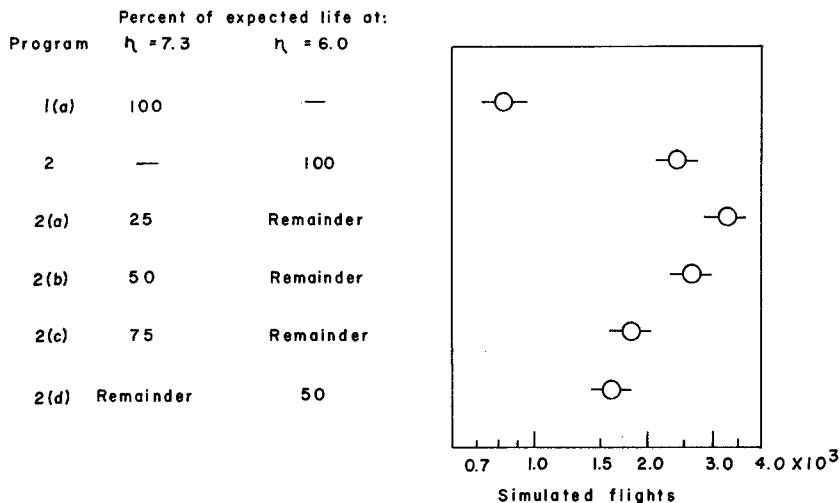
Figure 5.- Variable \eta test results. Maneuver load spectrum; 7075-T6 aluminum alloy.
