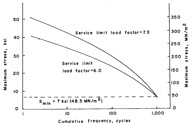
Figure 1.- Maneuver load cumulative frequency statistics.
