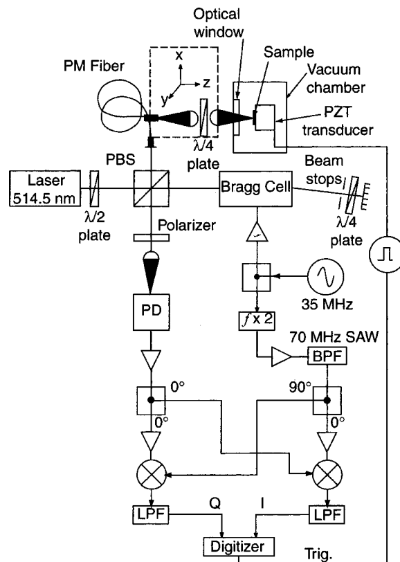
FIG. 2. Schematic diagram of the scanning laser Doppler vibrometer microscope (LDVM) system and associated demodulation setup. Notation: PBS, polarizing beam splitter; PM, polarization maintaining fiber; PD, photodetector; f \times 2 , frequency doubler; BPF, band pass filter; SAW, surface acoustic wave; and LPF, low pass filter.
