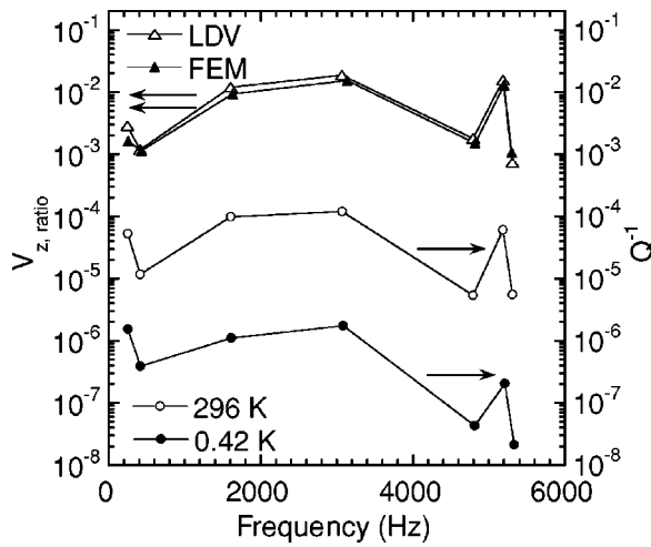
FIG. 3. Comparison of the measured (LDV) and calculated (FEM) nondimensional root integrated velocity ratio, V_{z, \text{ratio}} , for all observed modes with measured internal friction. The LDV data and FEM calculations are plotted with respect to the left axis while the internal friction is referenced to the right axis.
