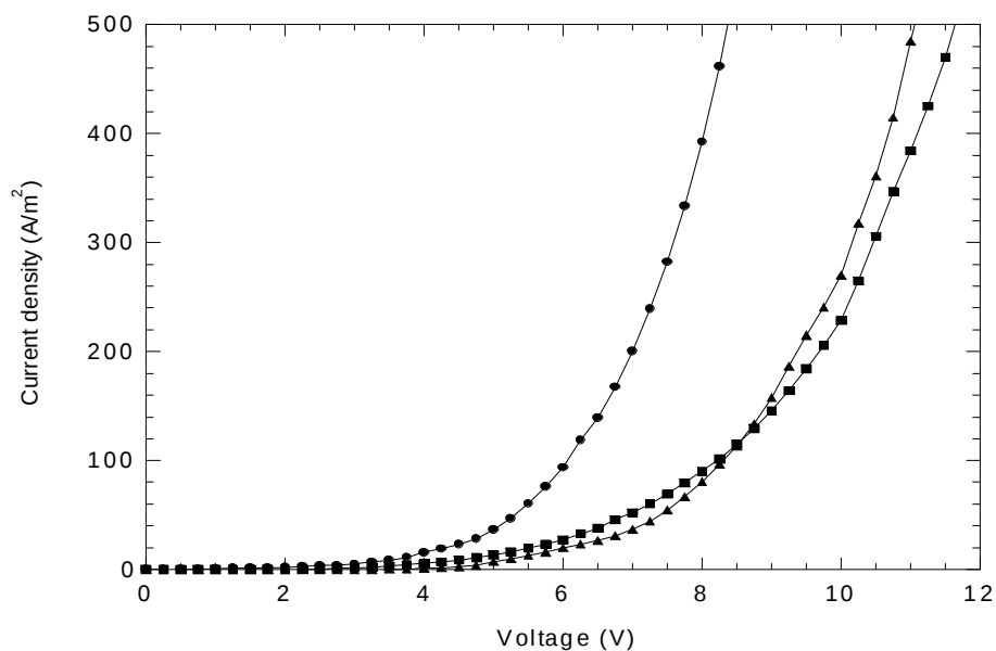
Figure 7. Current density versus voltage characteristics for devices with a PyPySPyPy (closed circles), a PPSP (closed squares) and a 2PSP (closed triangles) emissive/electron transport layer.
