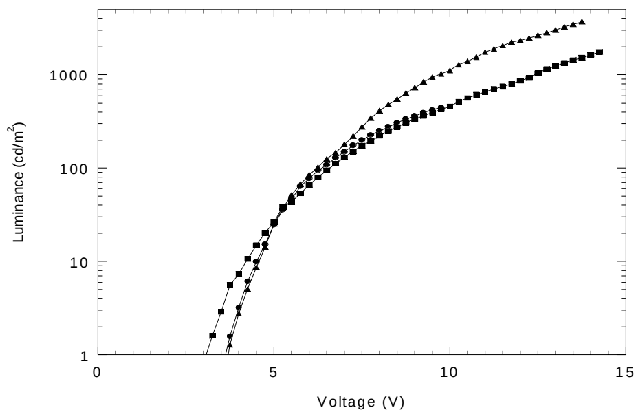
Figure 8. Luminance versus voltage characteristics for devices with a PyPySPyPy (closed circles), a PPSP (closed squares) and a 2PSP (closed triangles) emissive/electron transport layer.
