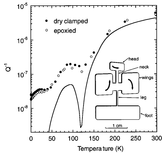
FIG. 1. The measured internal friction of the double paddle oscillator (points) compared to theory (solid line), Eq. (2). The pronounced dip predicted at 120 K is a result of a sign change in \alpha . This is only weakly observed experimentally due to contributions from yet unexplained sources of damping.
