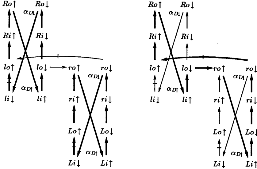
Figure 2: Critical cycles through the graph of a three-stage lap FIFO. The two graphs are identical; the sets of connected, bold arcs represent the critical cycles. An arc with a tick mark has \varepsilon = 1 . All other arcs have \varepsilon = 0 .
