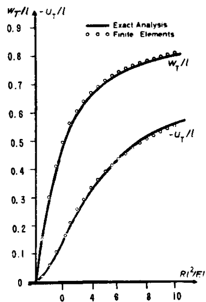
Figure 35. Cantilever Beam under Transverse Load
