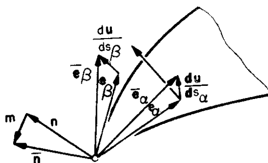
Figure 27. Change of Normal Vector due to Deformation
