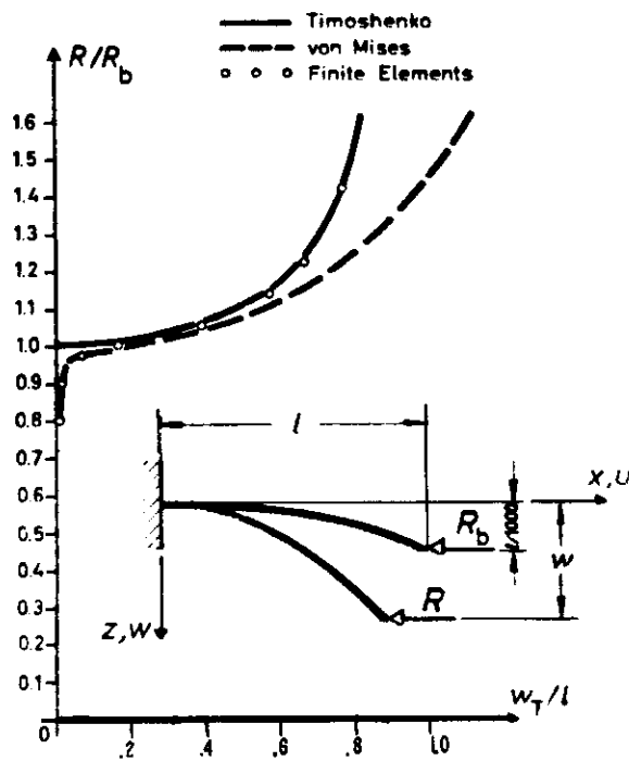
Figure 36. Beam with Initial Curvature
