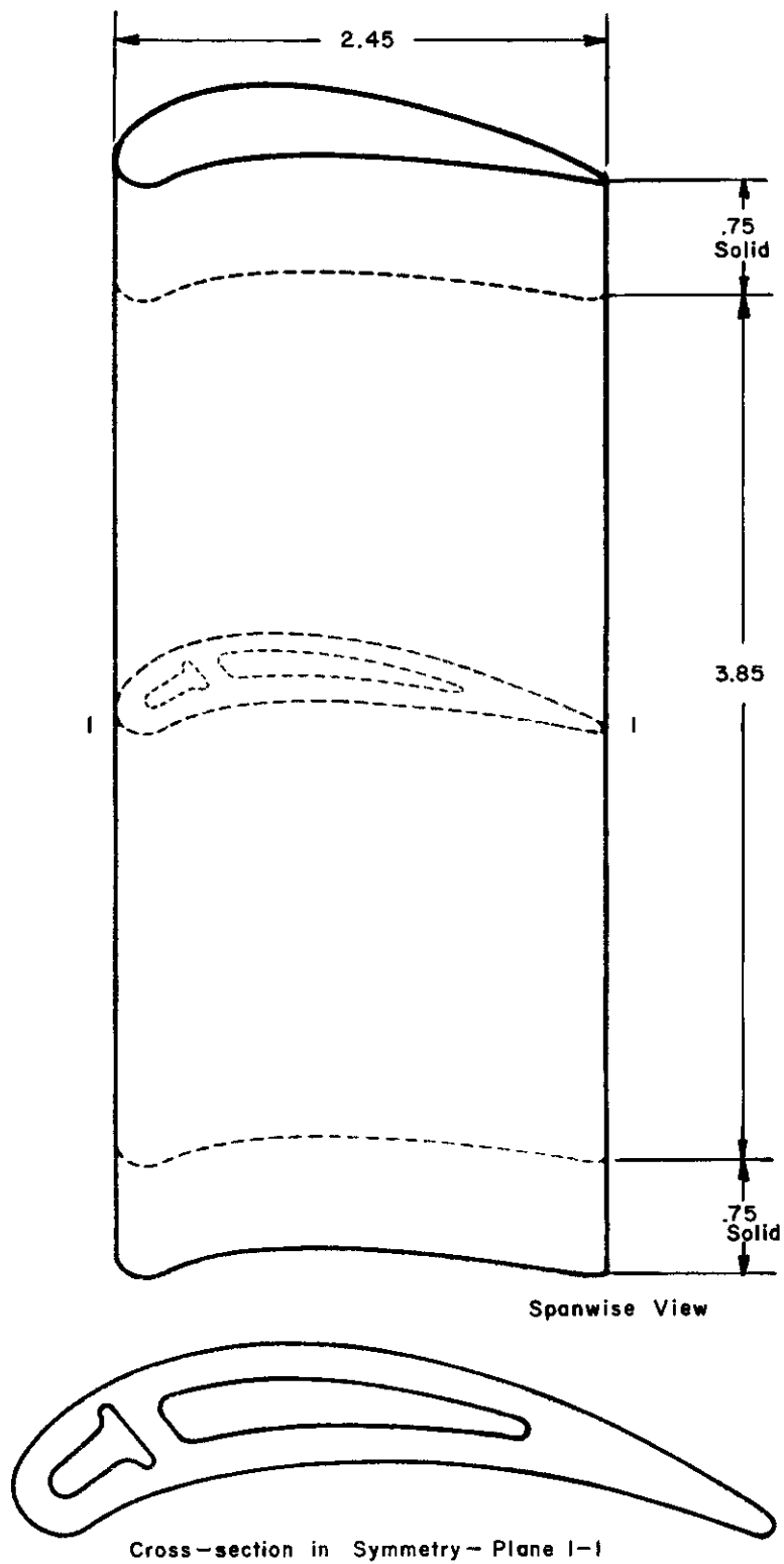
Figure 9. Turbine Vane
