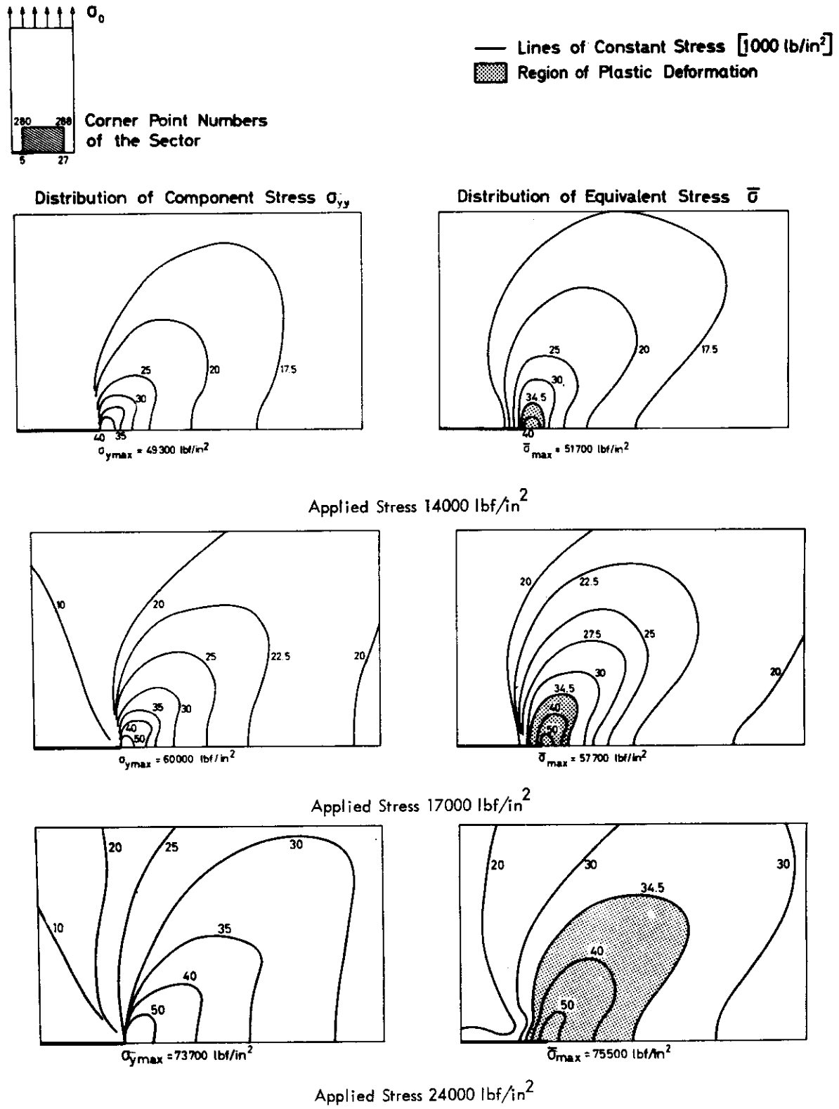
Figure 32. Plate with Crack
