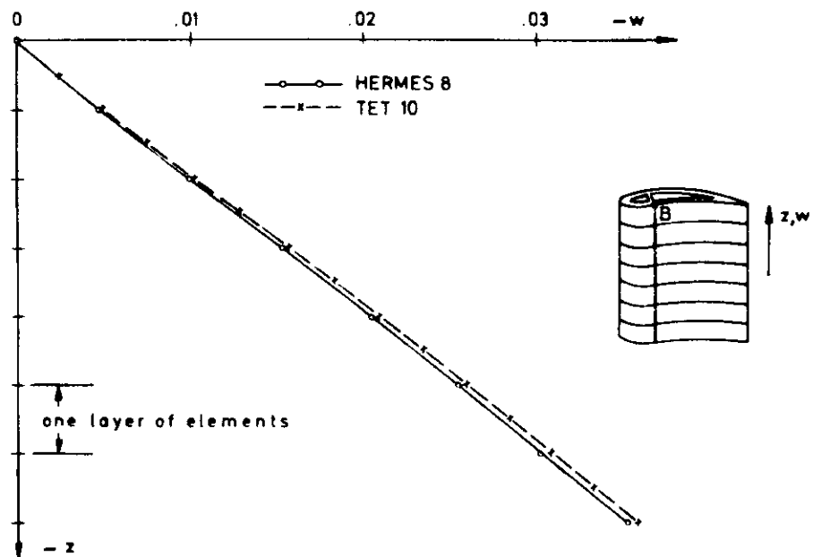
Figure 13. Comparison of Displacement w - TET 10 and HERMES 8 Analyses
