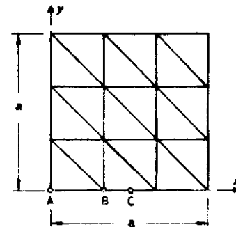
Idealisation of Simply Supported Quadratic Plate
