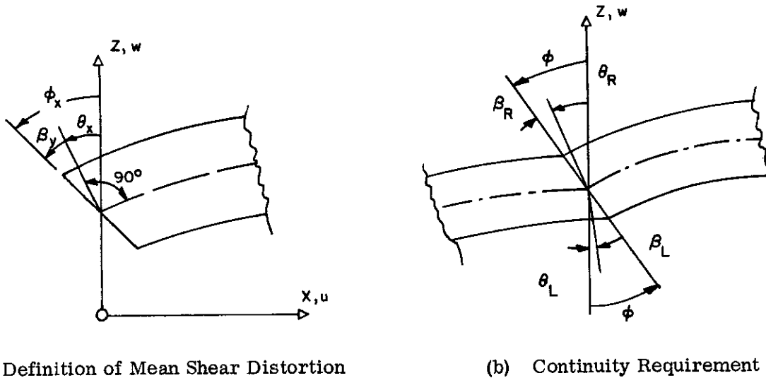
Figure 4. Shear Distortion Geometry
