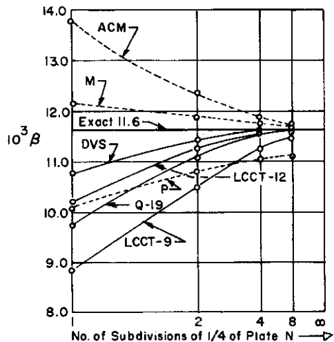
(c) Central Deflection w = \beta P a^2/D of Simply Supported Square Plate Under Concentrated Central Load P
