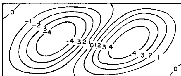
(D) Simply Supported Rectangular Plate ( 8/A = 0.4 ) Under Pure Shear
