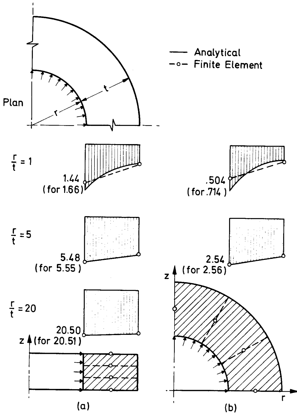
Figure 9. Lamé Solution for Hoof Stresses (a) Cylinder Under Uniform Internal Pressure (b) Sphere Under Uniform Internal Pressure
