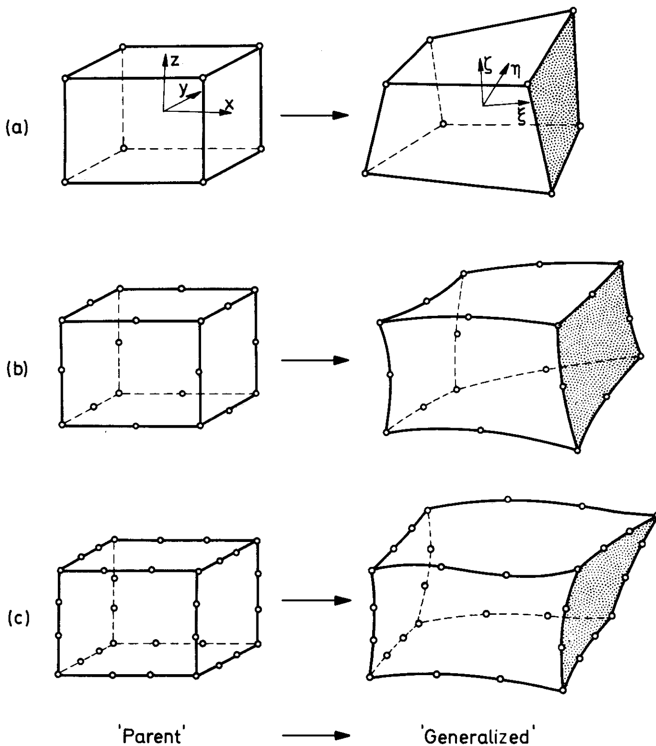
Figure 2. Three Dimensional, Hexadhedron, Family
