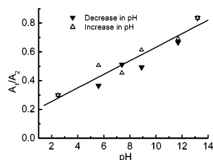
Figure 4. Normalized absorbance of the S_{11} band, plotted as the ratio A_1/A_2 of the peaks S_{11} and S_{22} of an as-treated SWNT sample (5-min sonication), reversibly responds to the pH change. 15
