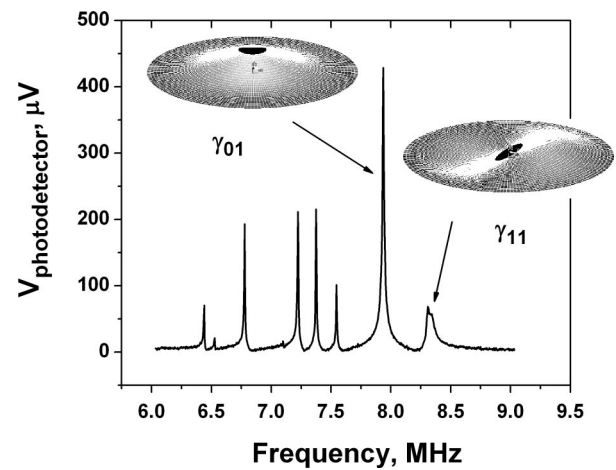
FIG. 3. Spectrum of the fundamental modes of the bare dome resonator acquired using \text{Ar}^+ laser drive and interferometric (HeNe laser) detection (all-optical operation). The modes of vibrations (see insets) were identified by varying the relative positions of the two laser beams and analyzing the spatial pattern of the phase difference between the driving signal and the detected mechanical motion. Multiple peaks corresponding to identical modes of vibrations but with different spatial orientation are observed due to slight asymmetry in the geometry of the dome. The highest quality factor ( Q \sim 10\,000 ) was exhibited by the \gamma_{01} mode.
