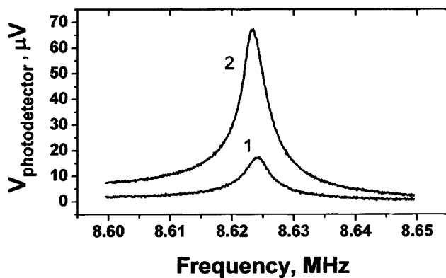
FIG. 4. Resonant peak corresponding to the \gamma_{01} mode of the vibrations of the dome acquired by microheater actuation with ac excitation power P_{ac} = 10 \mu\text{W} and dc power offset P_{dc} = 12 \mu\text{W} for resonance 1 and P_{dc} = 200 \mu\text{W} for resonance 2. Peak shift caused by dc heating corresponds to the tuning rate -3 \text{ Hz}/\mu\text{W} .
