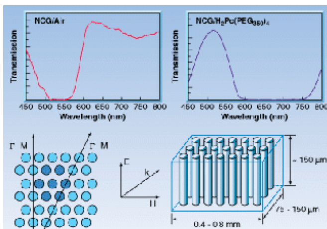
FIGURE 2. Photonic crystal based on nanochannel glass (NCG) in which the channels are filled with air has the transmission spectrum shown at left when measured along the high-symmetry \Gamma -M direction. In this case, a bandgap occurs between 510 and 560 nm—the reflectivity is high and the transmission can drop as low as 10^{-4} . If the channels are filled with an index-matched phthalocyanine (Pc) dye, this bandgap disappears. The spectrum now shows only the dye absorption between 580 and 770 nm (right). Inset shows typical structure of a photonic crystal based on nanochannel glass.
