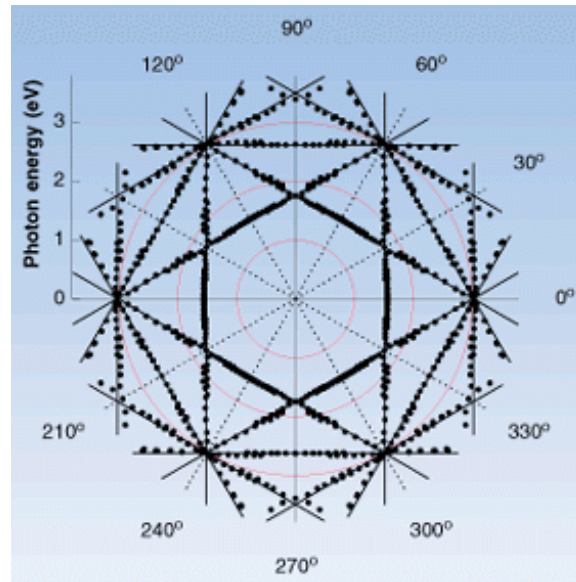
FIGURE 3. Polar plot shows attenuation positions (photonic bandgap energies) observed in a 2-D photonic crystal with periodicity of 280 nm. Near the G-M direction ( 0^\circ in this case), the energy of the first bandgap is not very sensitive to direction. This pattern of Brillouin zone boundaries is specific to the triangular lattice of the photonic crystal, a result reminiscent of x-ray analysis of the structure of ordinary crystals.
