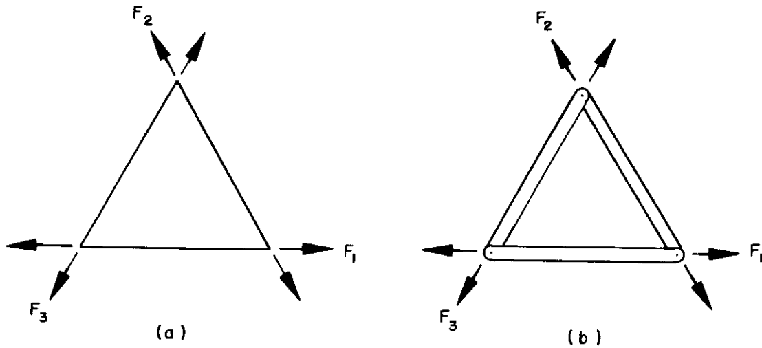
Figure 14. Equilateral Triangular Element
