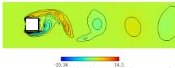
Fig. 3-11 Vorticity component \omega_z distribution around D/H=1.0 cylinder ( t=371 )
