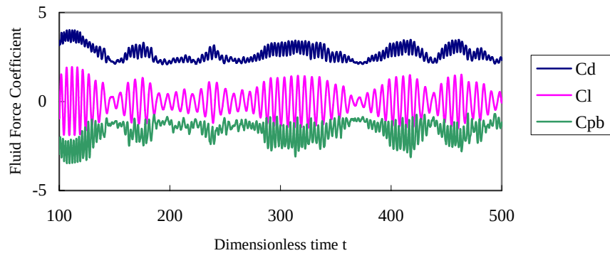
Fig. 3-7 Time history of fluid force of D/H=0.6 cylinder
