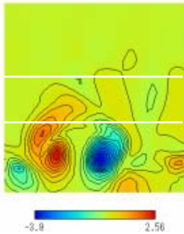
Fig. 4-3 Streamwise vorticity component \omega_x distribution behind D/H=0.4 cylinder (High pressure mode, x=3.2H , t=226 )
