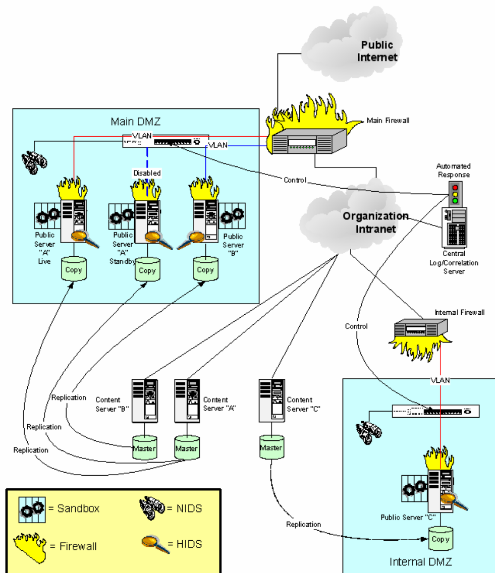
Figure 3 - Target Architecture
