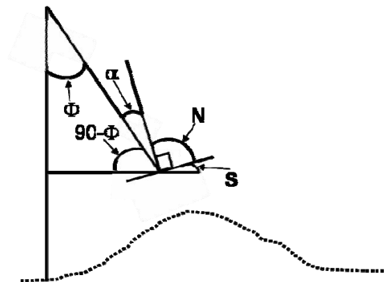
Figure 3.6 Schematic showing how \alpha , the angle between the center of the beam width and the normal to the local seafloor slope is found from \Phi_{old} and S.
